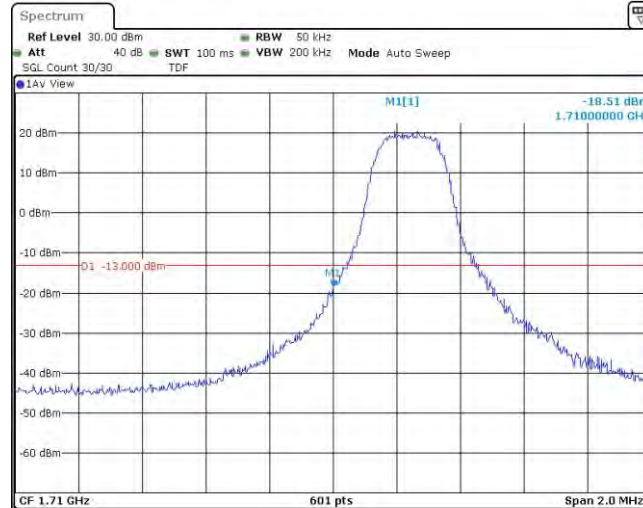
Band4-3MHz-16QAM-19965-1RB#14
