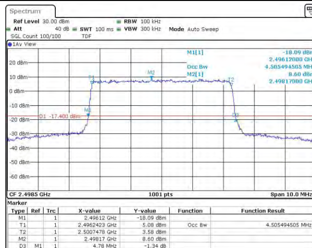
Band41-5MHz-16QAM-39675-25RB#0
