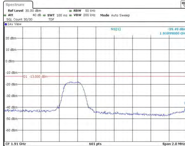
Band2-3MHz-16QAM-19185-1RB#14
