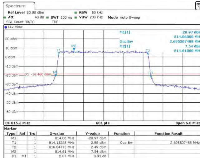
Band26-3MHz-16QAM-26705-15RB#0
