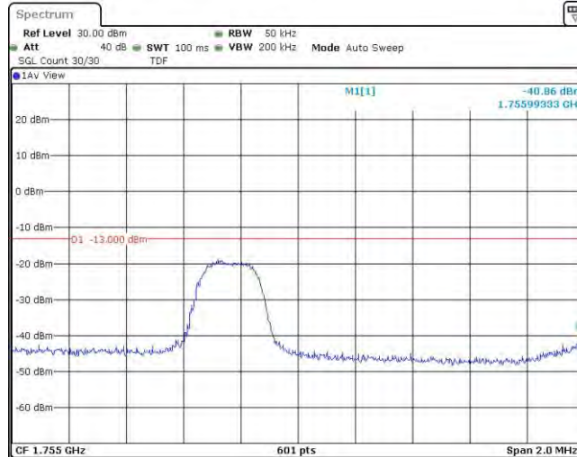
Band4-3MHz-QPSK-20385-1RB#14
