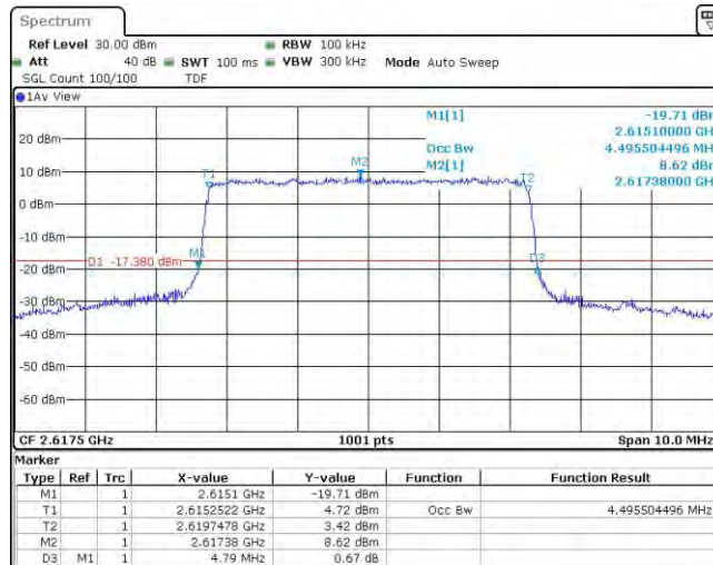
Band38-5MHz-16QAM-38225-25RB#0
