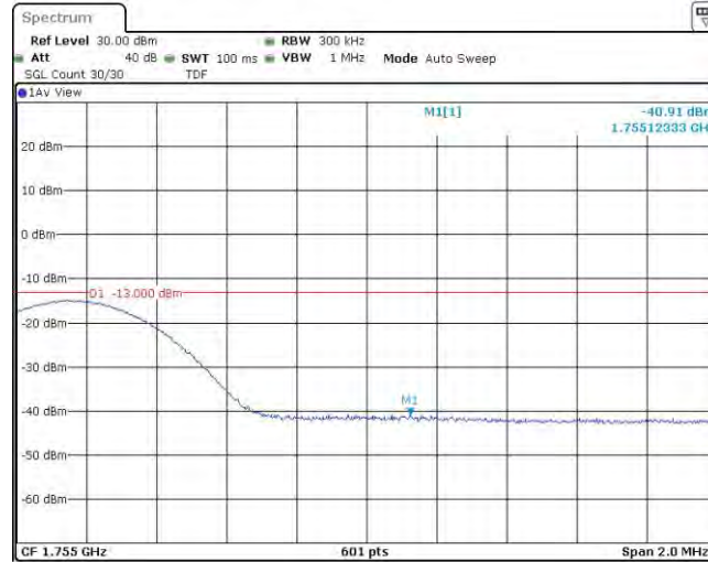
Band4-15MHz-QPSK-20325-1RB#74
