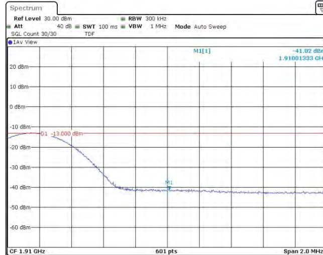
Band2-15MHz-QPSK-19125-1RB#74
