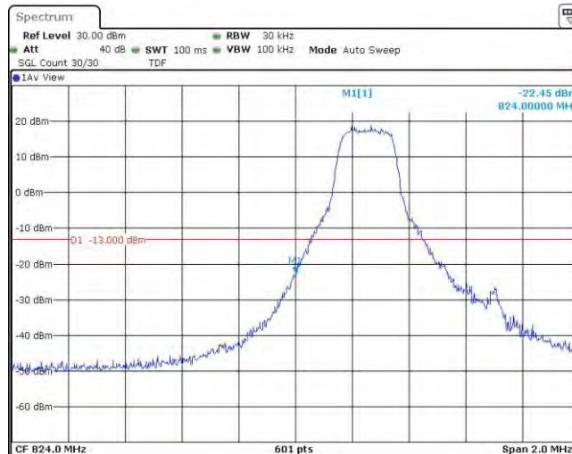
Band5-1.4MHz-QPSK-20407-1RB#5
