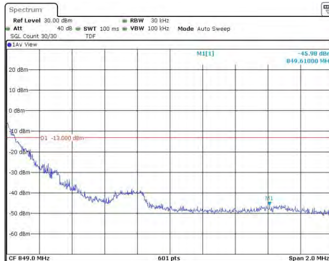
Band5-1.4MHz-QPSK-20643-1RB#5
