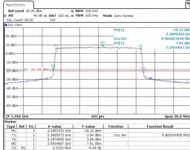
Band41-10MHz-QPSK-41540-50RB#0
