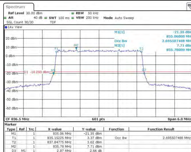
Band26-3MHz-16QAM-26915-15RB#0
