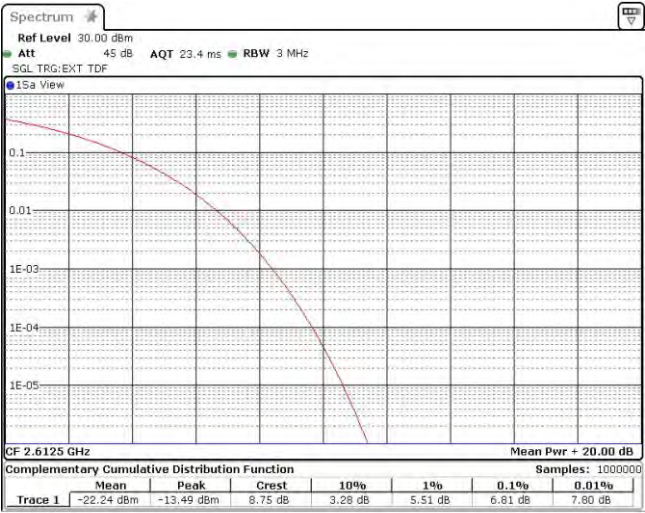
Band38-15MHz-QPSK-38175-75RB#0
