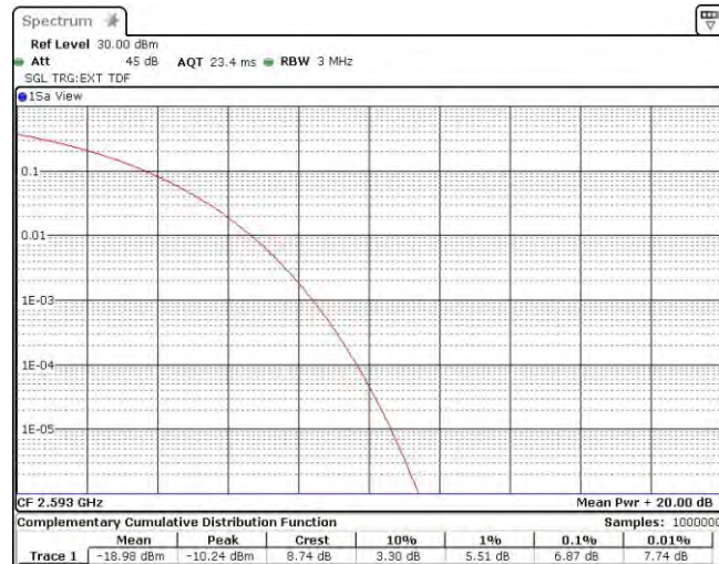
Band41-15MHz-16QAM-41515-1RB#0
