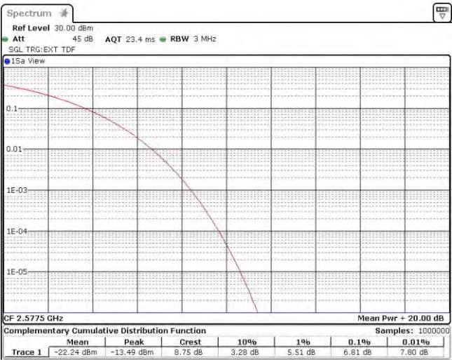
Band38-15MHz-QPSK-37825-75RB#0
