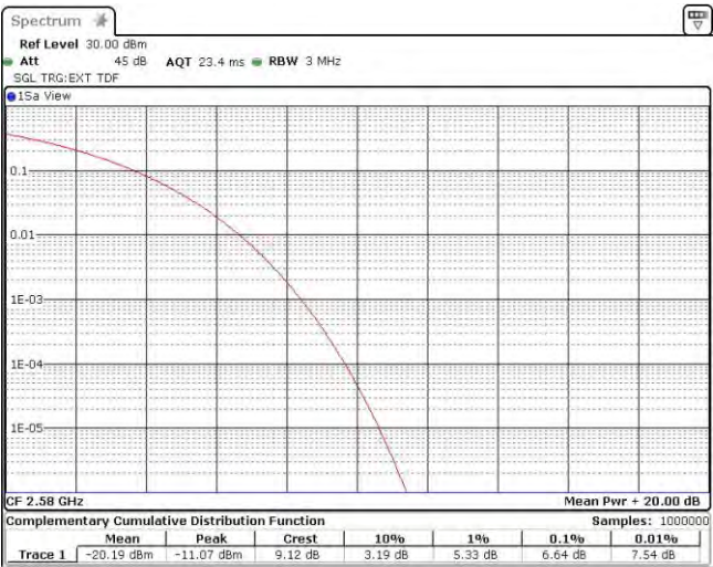
Band38-20MHz-QPSK-37850-100RB#0
