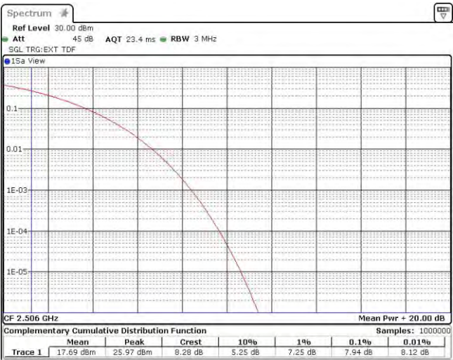
Band41-20MHz-QPSK-39750-100RB#0
