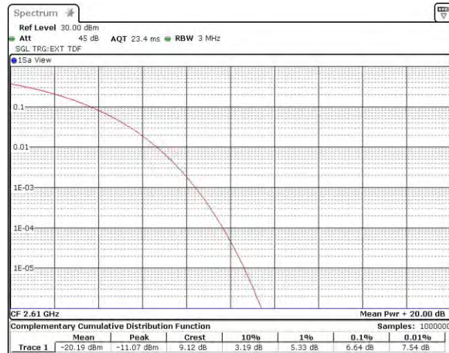
Band38-20MHz-16QAM-38150-100RB#0
