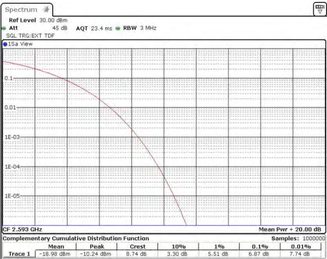
Band41-10MHz-QPSK-40620-50RB#0
