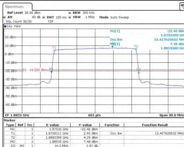
Band25-15MHz-16QAM-26365-75RB#0
