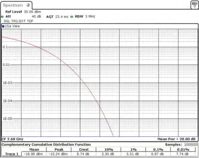
Band41-20MHz-QPSK-41490-100RB#0
