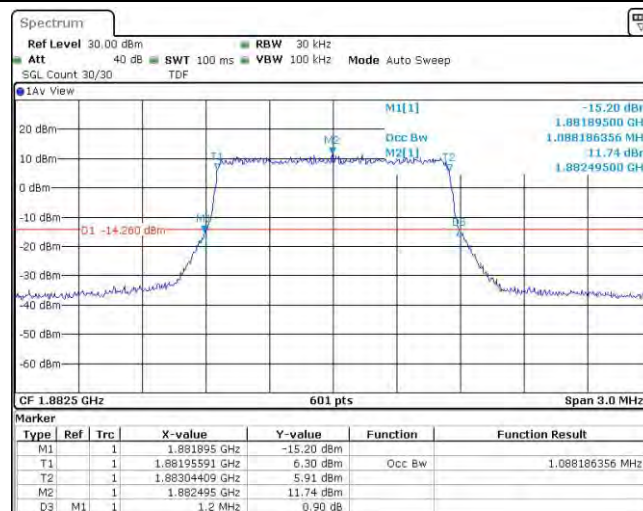
Band25-1.4MHz-16QAM-26365-6RB#0
