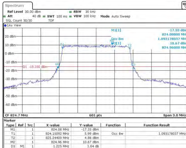
Band5-1.4MHz-QPSK-20525-6RB#0
