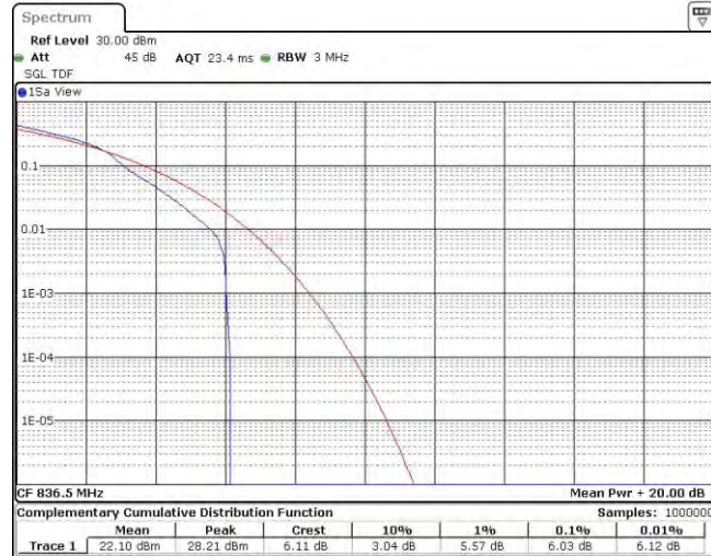
Band26-1.4MHz-16QAM-26915-6RB#0
