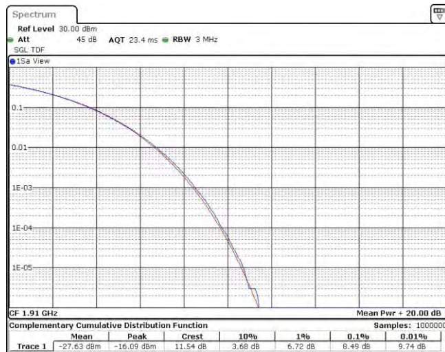
Band25-10MHz-16QAM-26640-50RB#0
