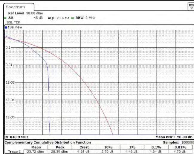
Band26-1.4MHz-QPSK-27033-6RB#0
