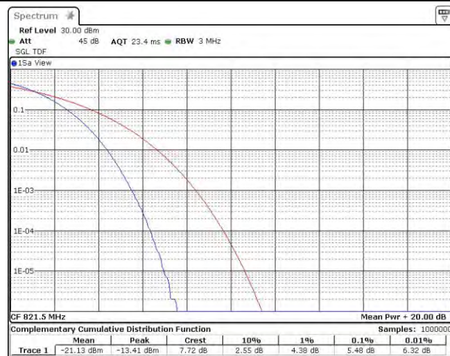
Band26-15MHz-QPSK-26765-75RB#0
