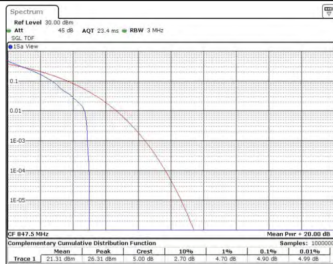
Band26-3MHz-QPSK-27025-15RB#0
