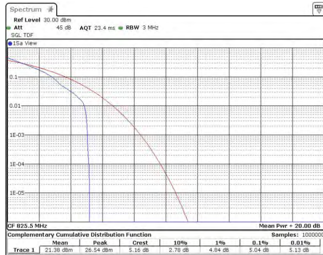
Band26-3MHz-QPSK-26805-15RB#0
