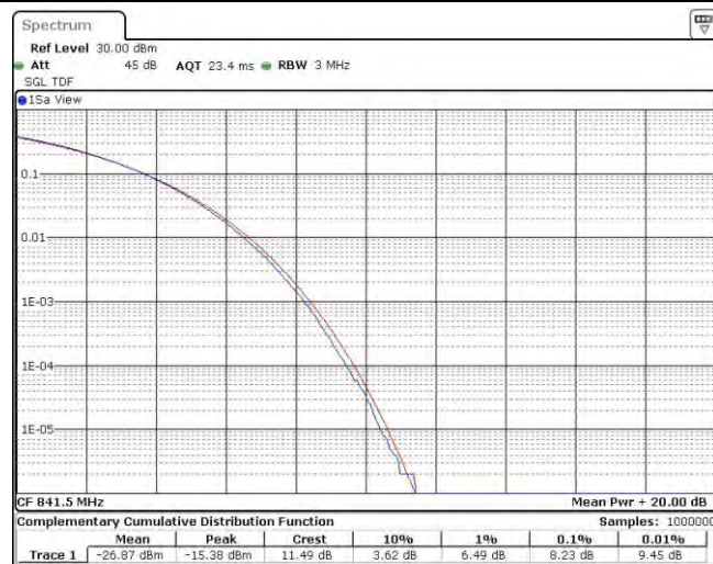
Band26-15MHz-QPSK-26965-75RB#0
