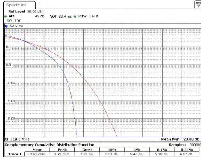
Band26-10MHz-16QAM-26740-50RB#0
