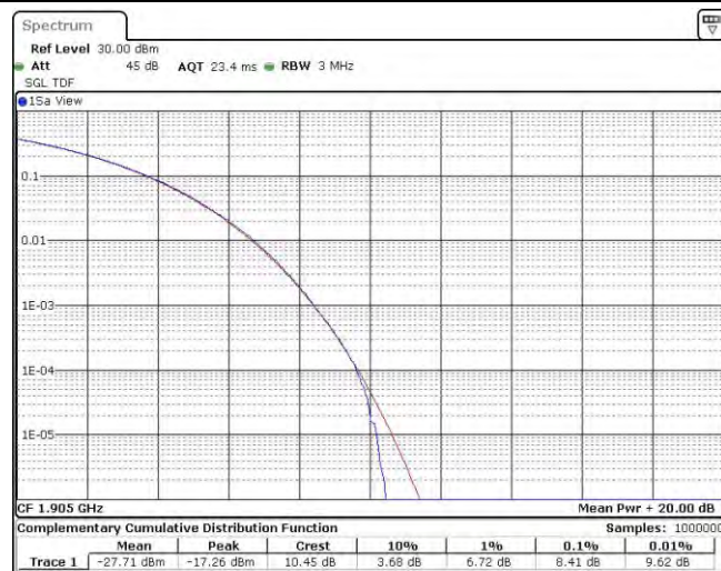
Band25-20MHz-16QAM-26590-100RB#0
