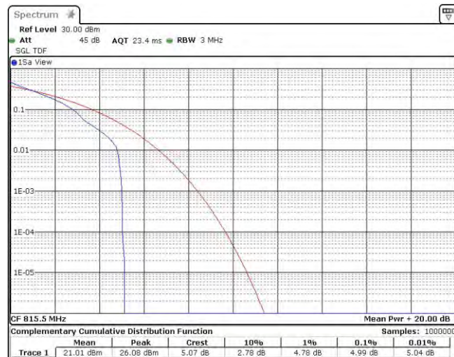
Band26-3MHz-QPSK-26705-15RB#0
