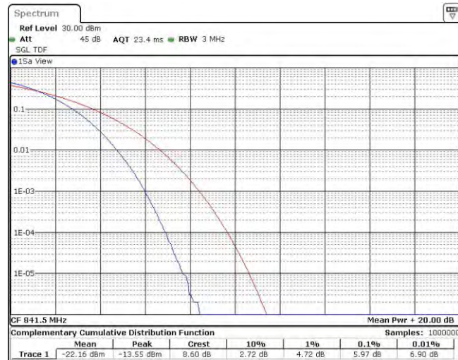
Band26-15MHz-16QAM-26965-75RB#0
