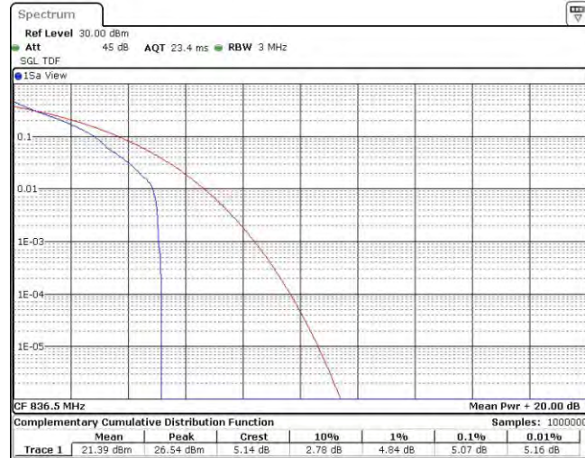
Band26-3MHz-QPSK-26915-15RB#0
