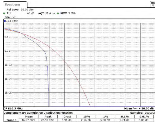
Band26-5MHz-16QAM-26715-25RB#0
