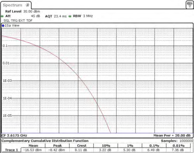
Band38-5MHz-16QAM-38225-25RB#0
