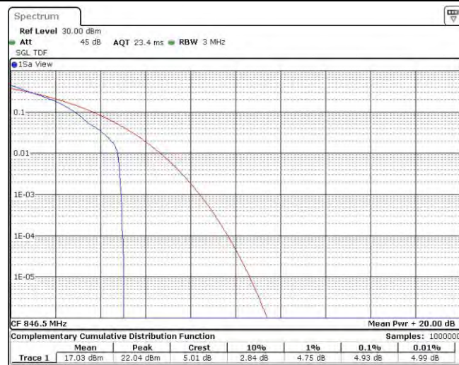
Band26-5MHz-QPSK-27015-25RB#0
