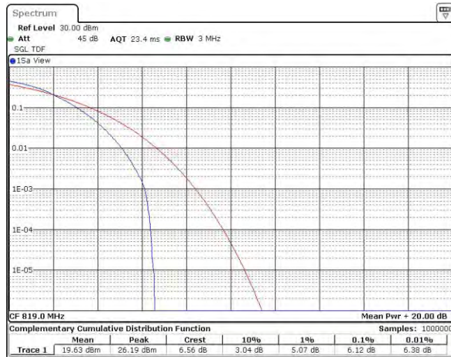
Band26-5MHz-16QAM-26765-1RB#0
