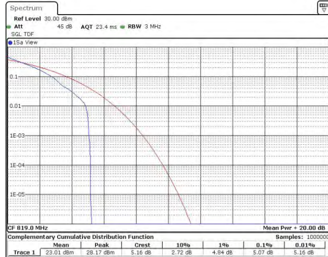
Band26-1.4MHz-QPSK-26740-6RB#0
