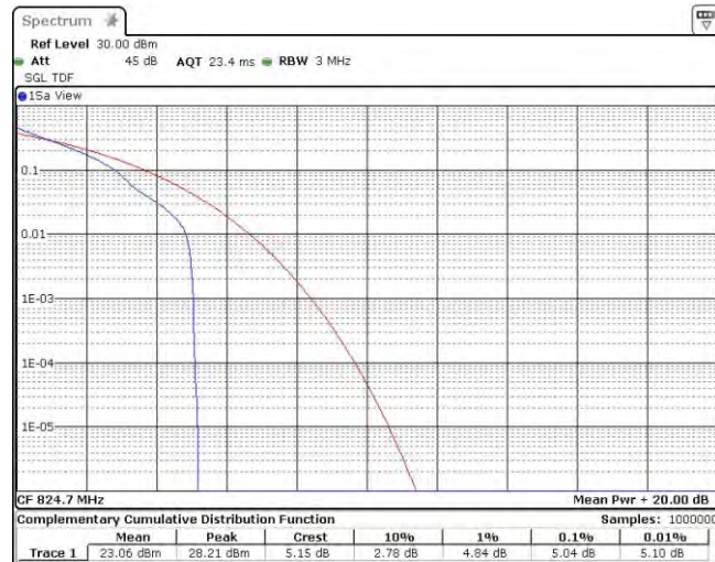
Band26-1.4MHz-QPSK-26797-6RB#0
