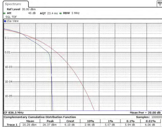
Band26-3MHz-16QAM-26915-15RB#0
