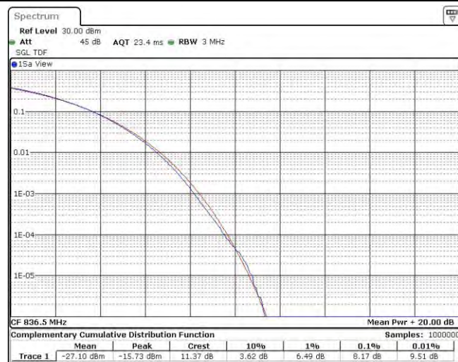
Band26-15MHz-16QAM-26915-75RB#0
