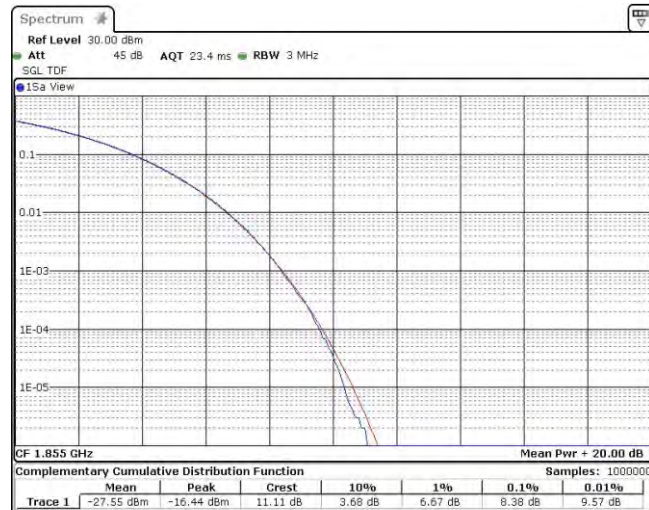
Band25-10MHz-QPSK-26090-50RB#0
