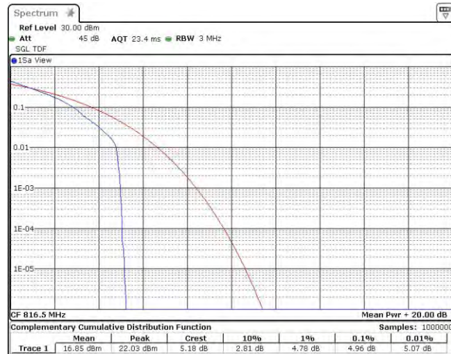
Band26-5MHz-QPSK-26715-25RB#0
