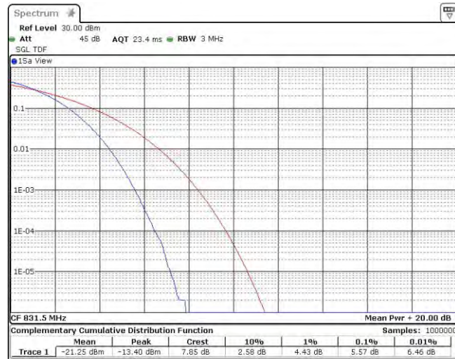
Band26-15MHz-QPSK-26865-75RB#0
