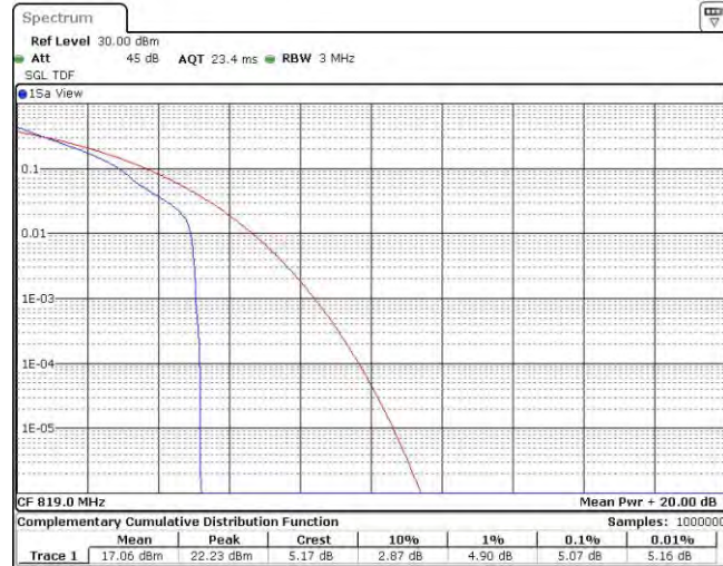
Band26-5MHz-QPSK-26740-25RB#0
