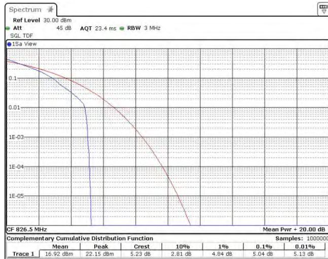
Band26-5MHz-QPSK-26815-25RB#0
