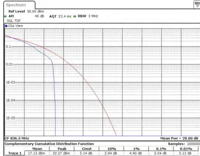
Band26-5MHz-QPSK-26915-25RB#0
