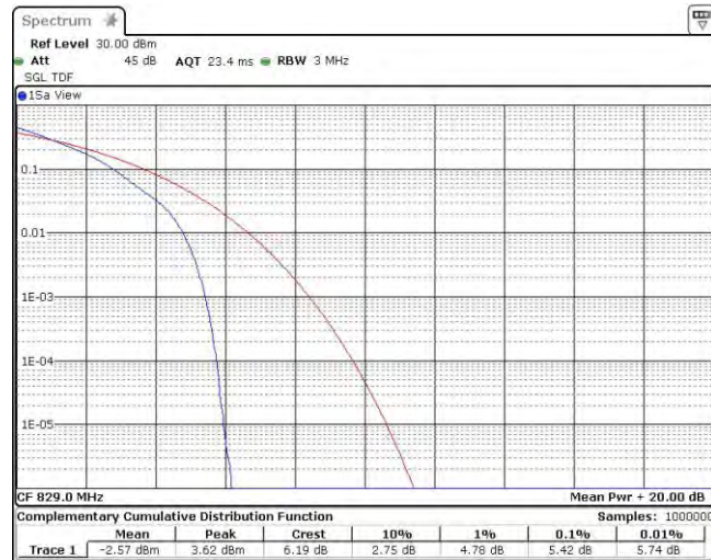
Band26-10MHz-QPSK-26840-50RB#0
