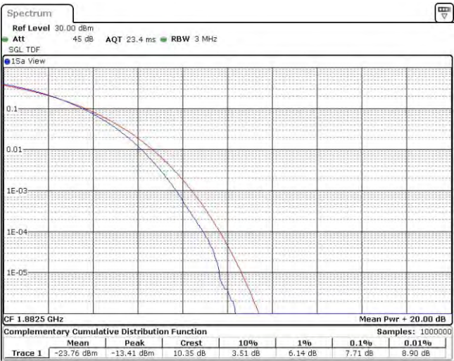
Band25-5MHz-16QAM-26365-25RB#0
