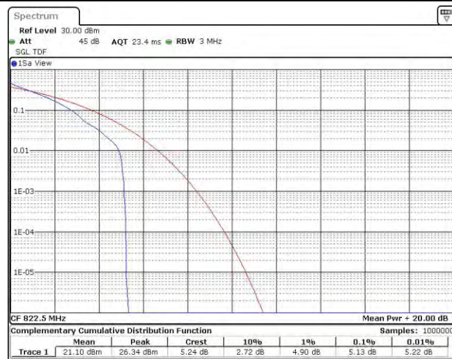
Band26-3MHz-QPSK-26775-15RB#0
