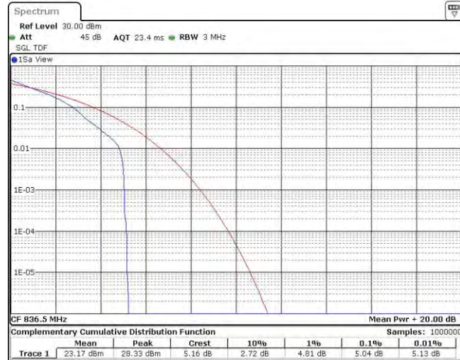
Band26-1.4MHz-QPSK-26915-6RB#0
