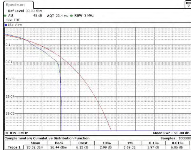
Band26-3MHz-16QAM-26740-15RB#0
