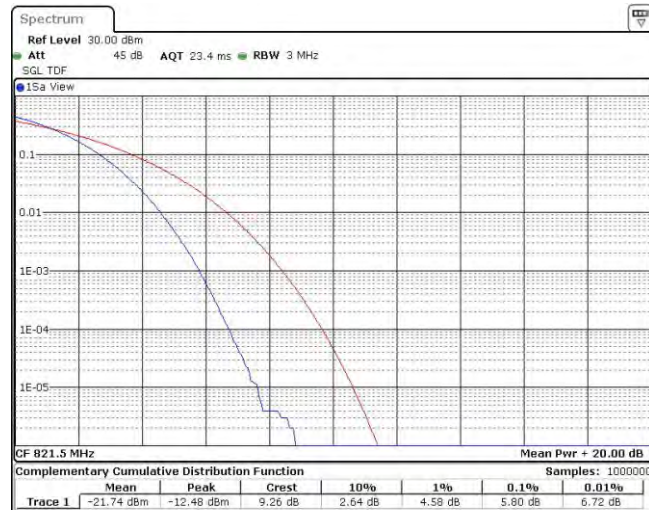
Band26-15MHz-16QAM-26765-75RB#0
