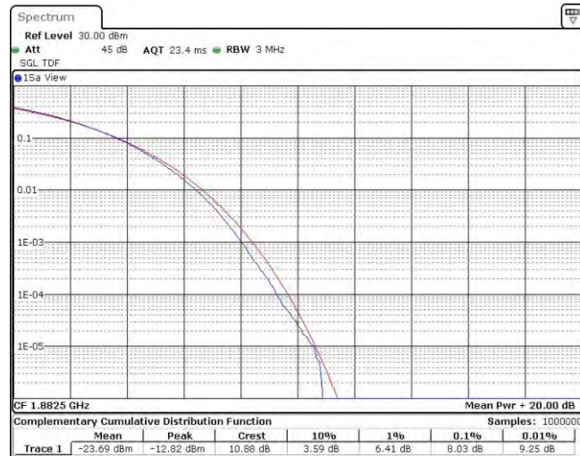
Band25-15MHz-16QAM-26615-1RB#0
