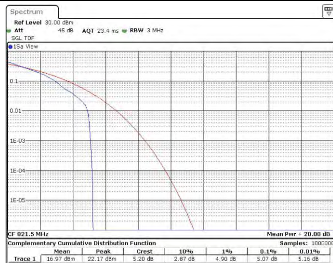
Band26-5MHz-QPSK-26765-25RB#0
