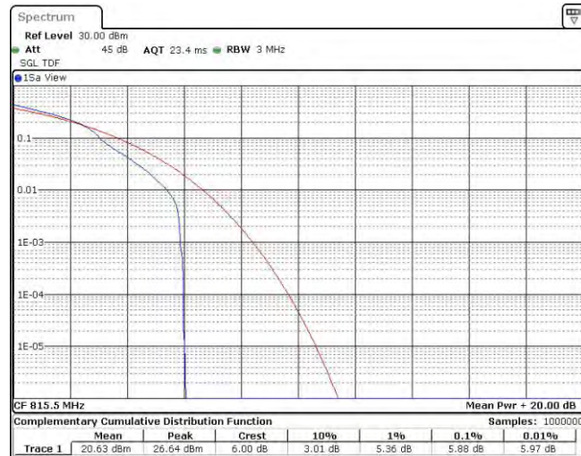
Band26-3MHz-16QAM-26705-15RB#0
