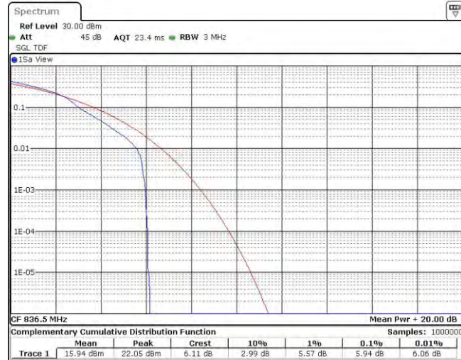
Band26-5MHz-16QAM-26915-25RB#0
