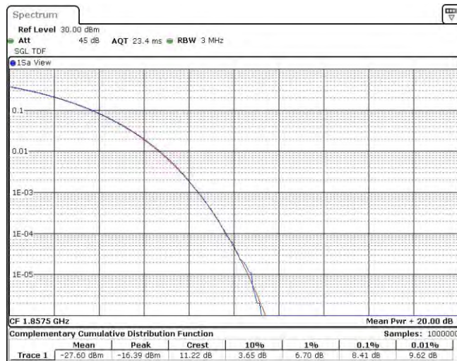
Band25-15MHz-16QAM-26115-75RB#0
