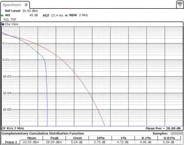
Band26-1.4MHz-QPSK-26697-6RB#0
