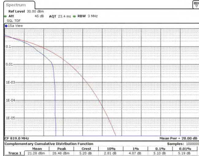
Band26-3MHz-QPSK-26740-15RB#0
