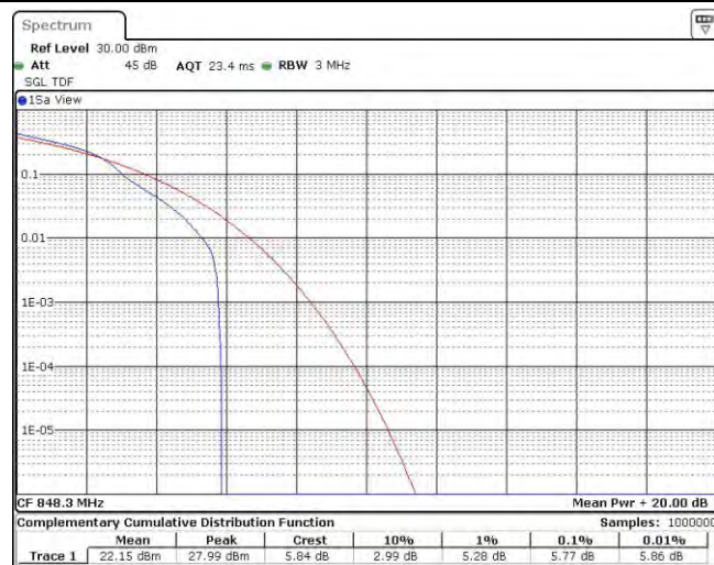
Band26-1.4MHz-16QAM-27033-6RB#0
