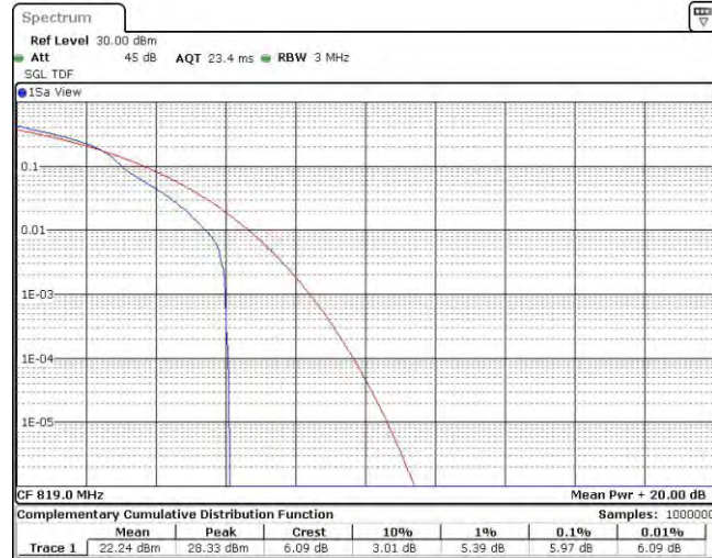
Band26-1.4MHz-16QAM-26740-6RB#0
