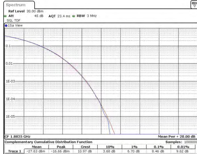
Band25-15MHz-16QAM-26365-75RB#0
