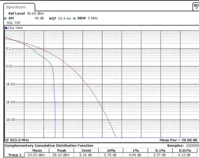
Band26-1.4MHz-QPSK-26783-6RB#0
