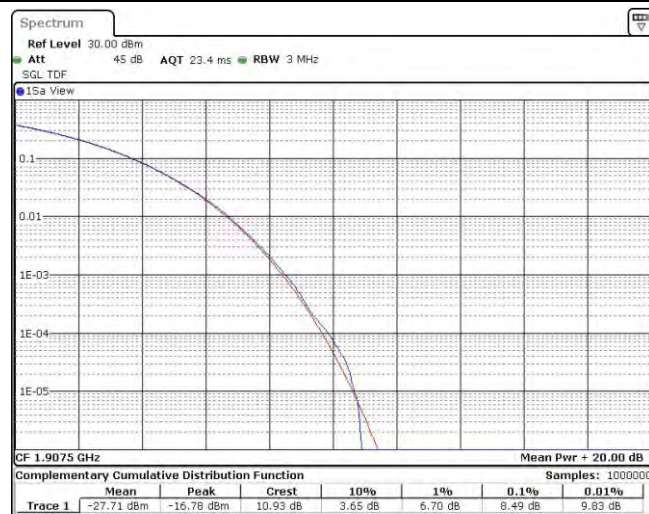
Band25-15MHz-QPSK-26615-75RB#0
