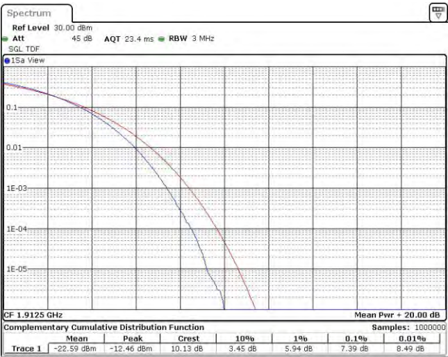
Band25-5MHz-16QAM-26665-25RB#0
