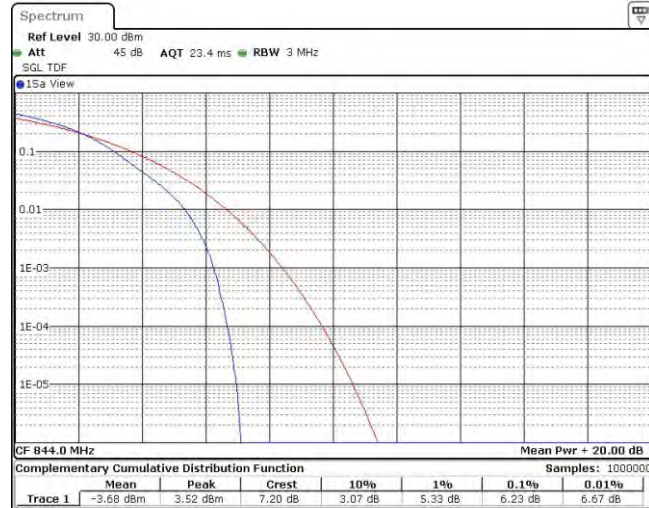
Band26-10MHz-16QAM-26990-50RB#0
