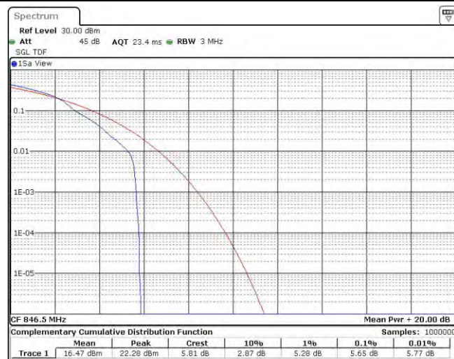
Band26-5MHz-16QAM-27015-25RB#0
