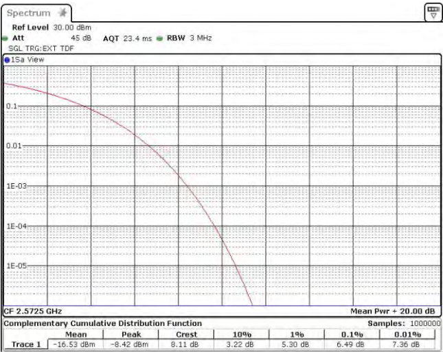
Band38-5MHz-QPSK-37775-25RB#0
