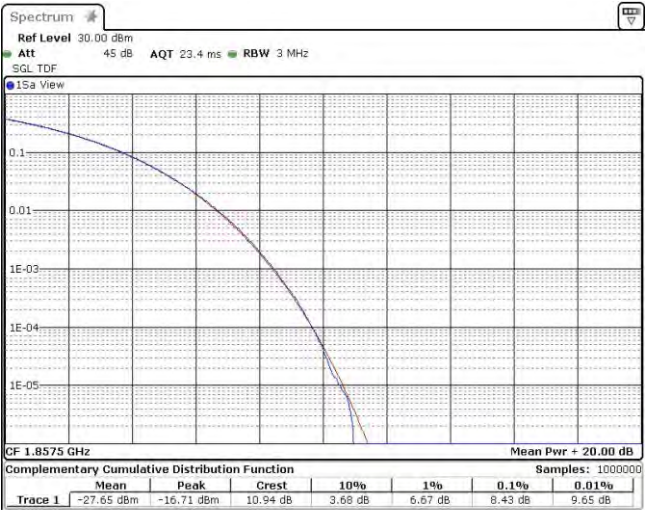
Band25-15MHz-QPSK-26115-75RB#0
