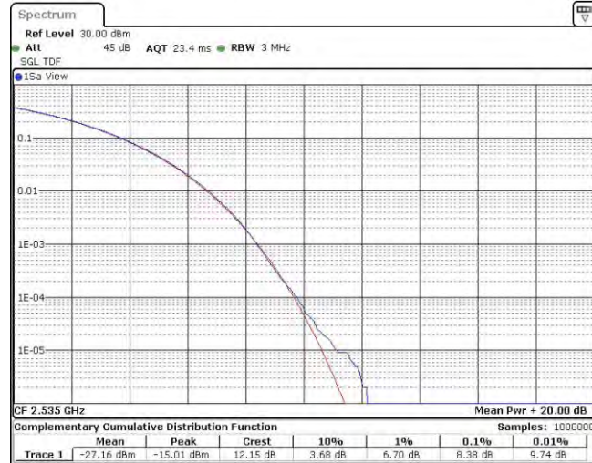
Band7-10MHz-16QAM-21100-50RB#0
