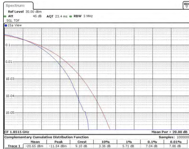
Band25-3MHz-16QAM-26055-15RB#0
