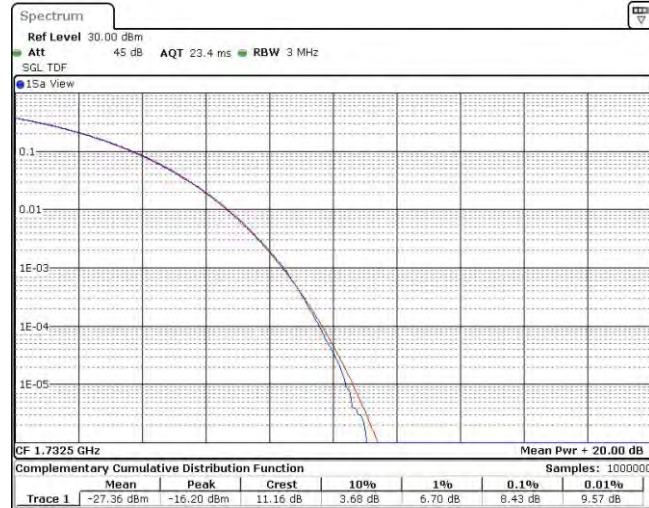
Band4-15MHz-16QAM-20175-75RB#0
