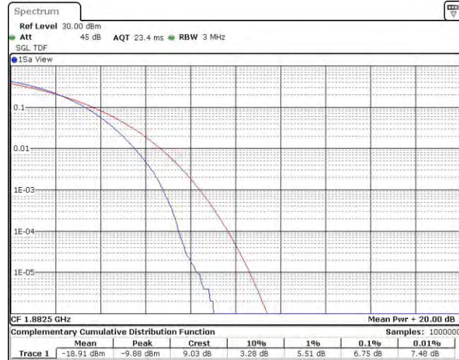
Band25-1.4MHz-16QAM-26365-6RB#0
