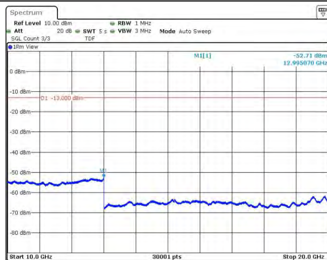
Band2-9262-3-10000~20000MHz
