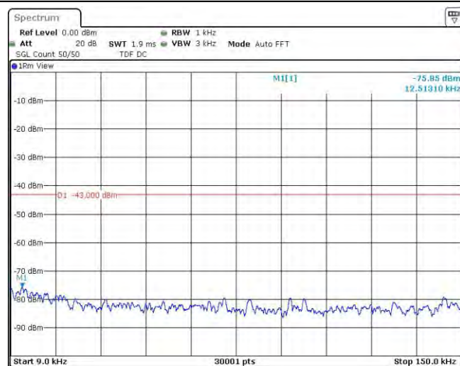
Band4-1513-1-0.009~0.15MHz
