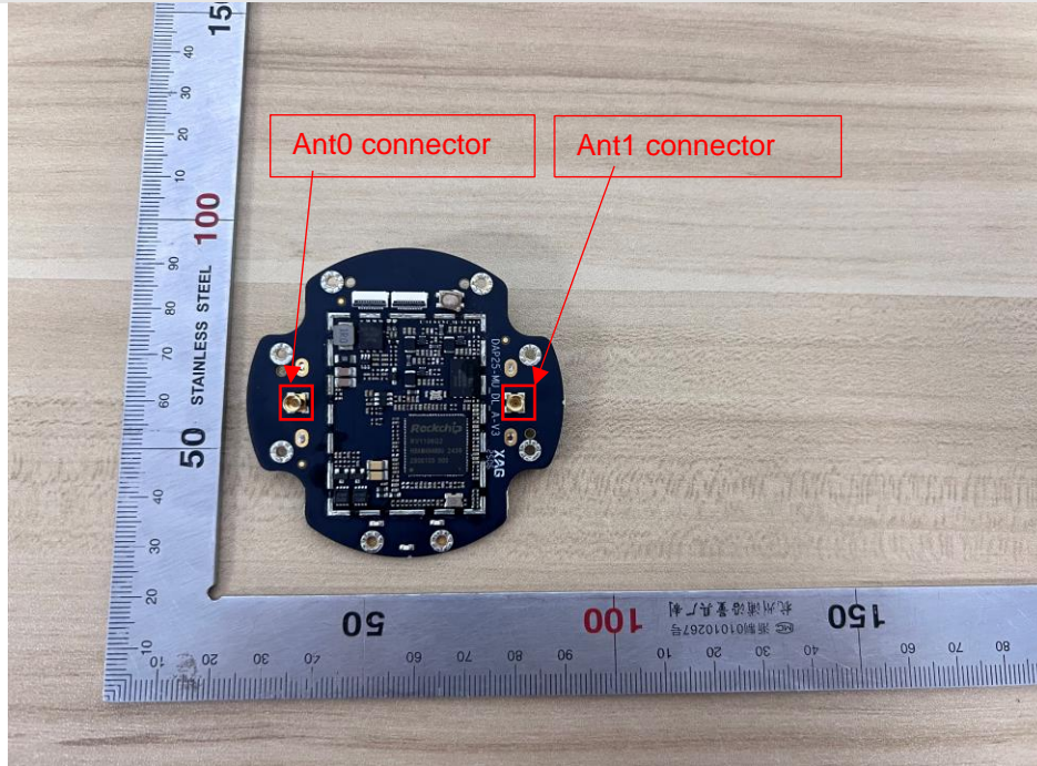
Internal View of EUT-7
