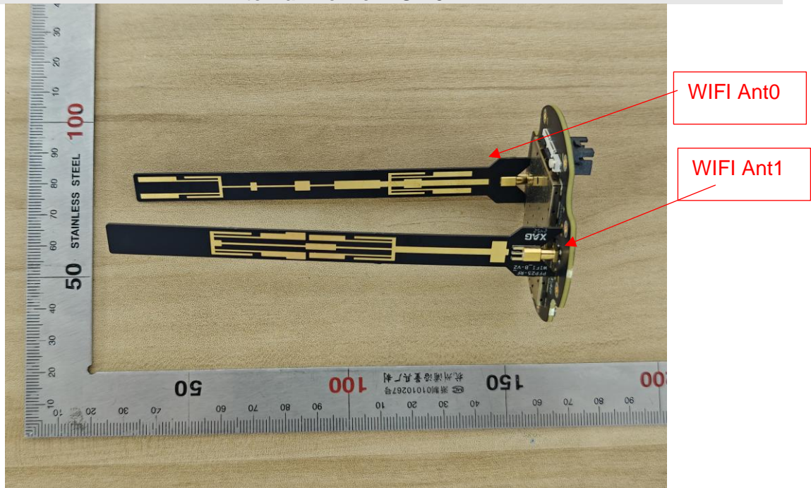
Internal View of EUT-8
