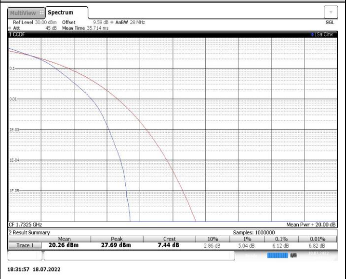
Band4-15MHz-16QAM-20175-75RB#0
