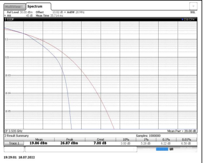
Band7-20MHz-16QAM-21100-100RB#0
