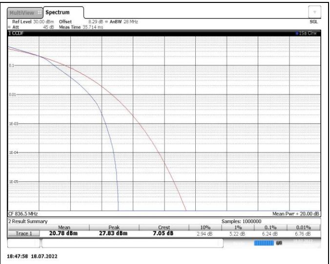
Band5-10MHz-16QAM-20525-50RB#0
