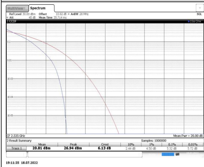
Band7-10MHz-QPSK-21100-50RB#0
