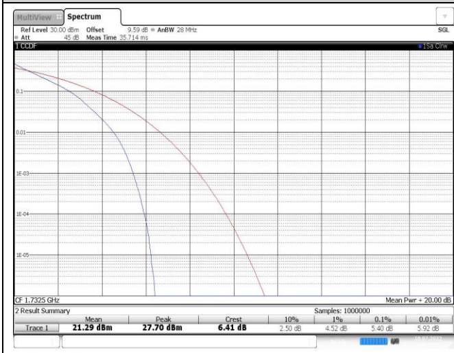
Band4-3MHz-QPSK-20175-15RB#0
