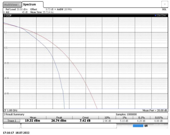
Band2-5MHz-16QAM-18900-25RB#0
