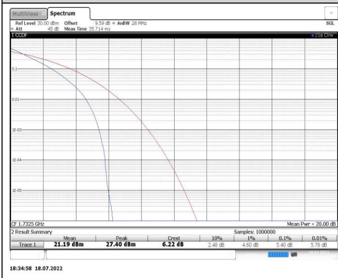
Band4-20MHz-QPSK-20175-100RB#0
