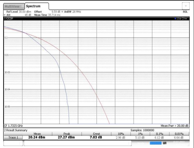
Band4-1.4MHz-16QAM-20175-6RB#0
