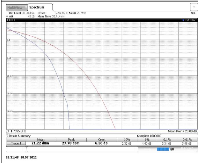
Band4-15MHz-QPSK-20175-75RB#0
