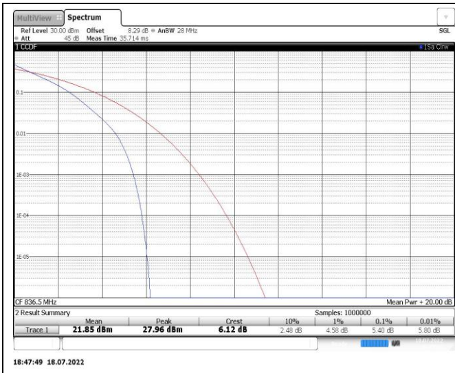
Band5-10MHz-QPSK-20525-50RB#0
