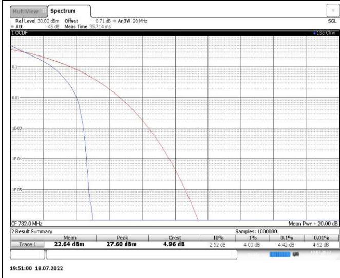
Band13-10MHz-QPSK-23230-50RB#0
