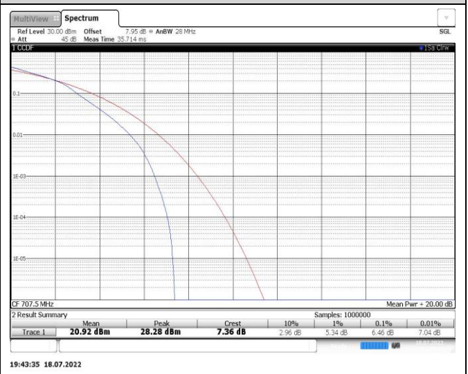
Band12-10MHz-16QAM-23095-50RB#0
