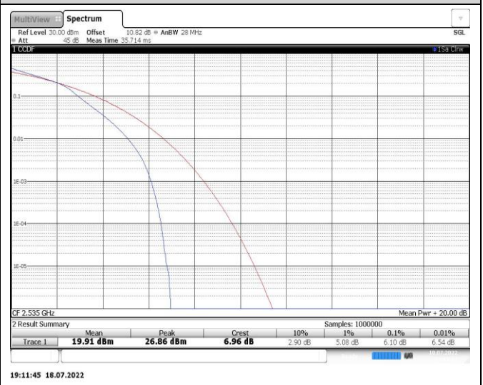
Band7-10MHz-16QAM-21100-50RB#0
