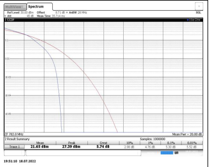
Band13-10MHz-16QAM-23230-50RB#0
