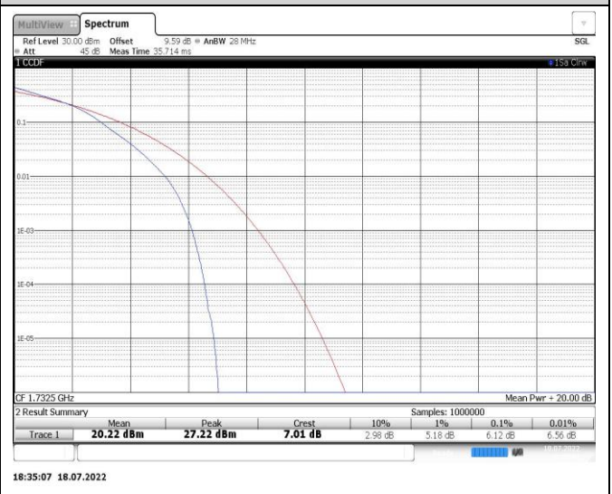
Band4-20MHz-16QAM-20175-100RB#0
