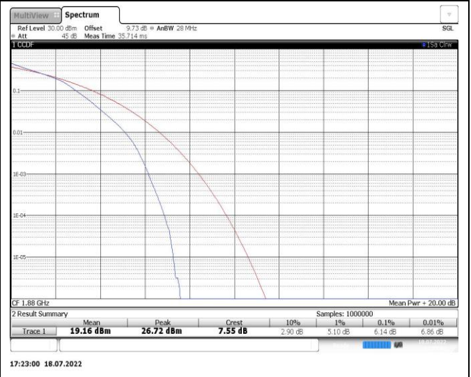
Band2-15MHz-16QAM-18900-75RB#0
