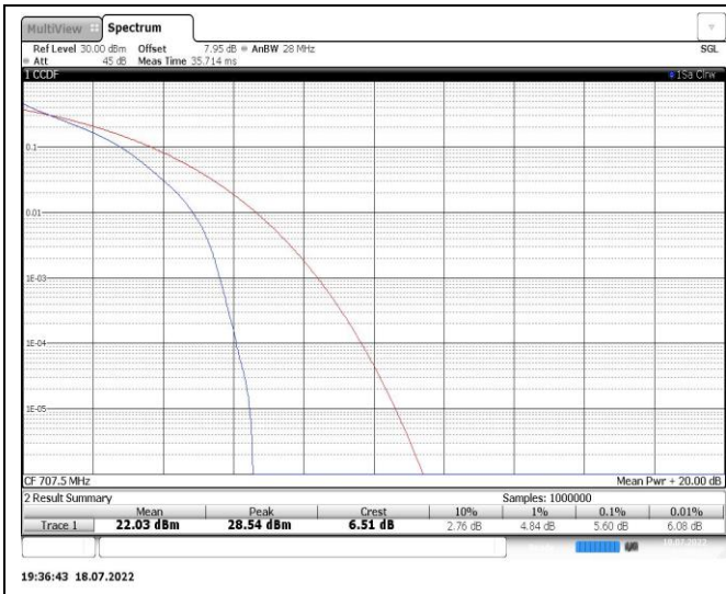
Band12-3MHz-QPSK-23095-15RB#0
