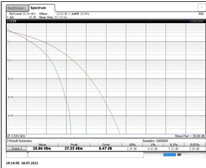
Band7-15MHz-QPSK-21100-75RB#0
