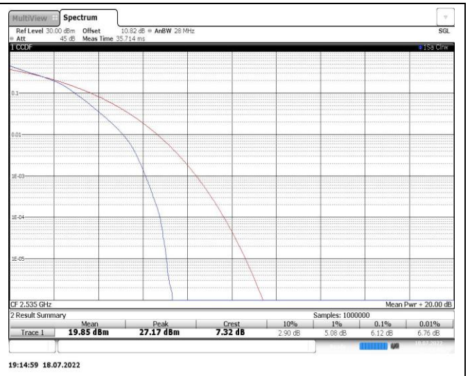
Band7-15MHz-16QAM-21100-75RB#0
