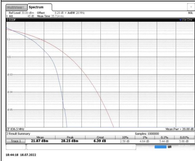
Band5-5MHz-QPSK-20525-25RB#0
