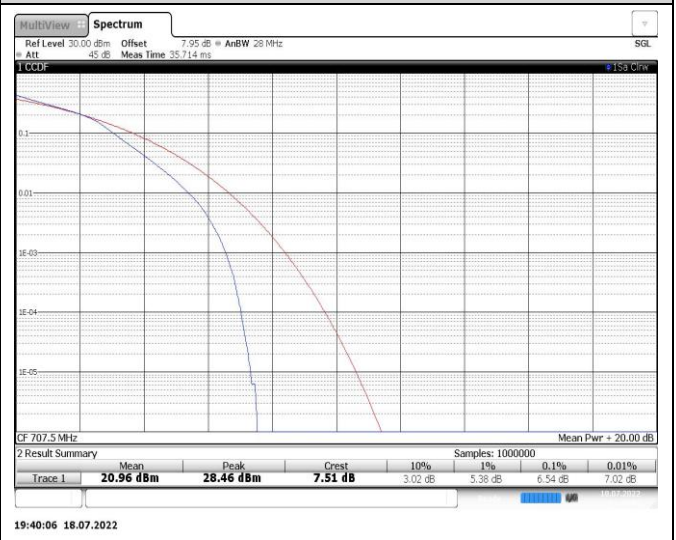
Band12-5MHz-16QAM-23095-25RB#0
