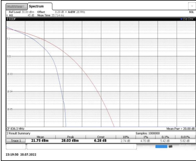
Band5-3MHz-QPSK-20525-15RB#0
