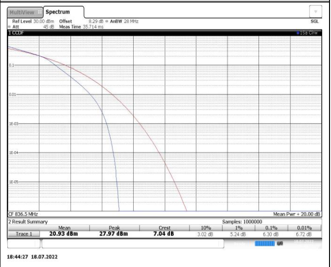
Band5-5MHz-16QAM-20525-25RB#0
