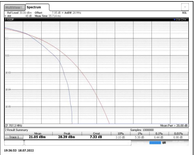
Band12-3MHz-16QAM-23095-15RB#0
