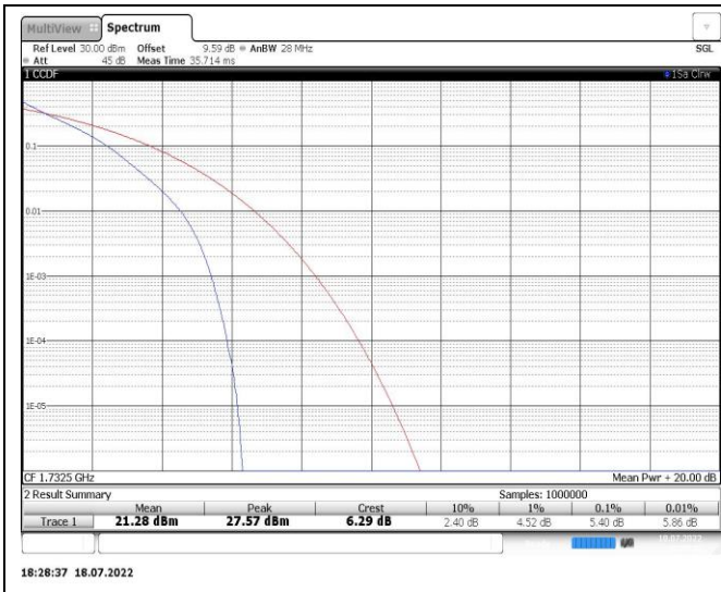
Band4-10MHz-QPSK-20175-50RB#0
