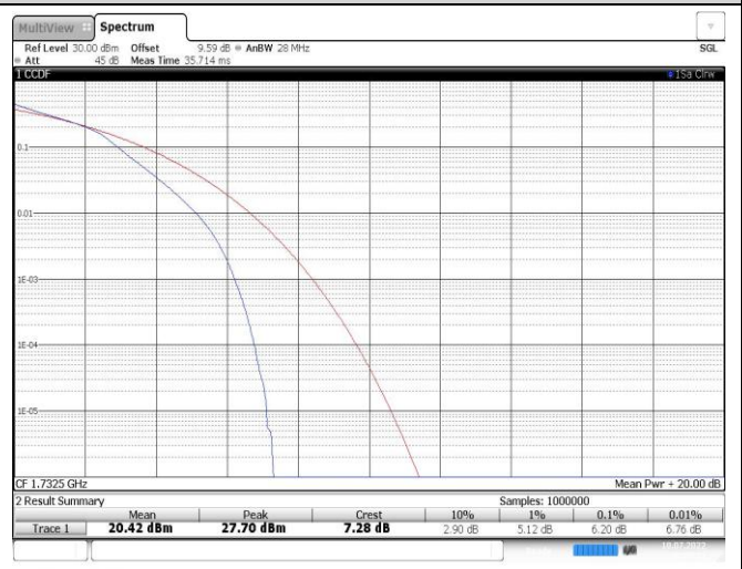
Band4-3MHz-16QAM-20175-15RB#0
