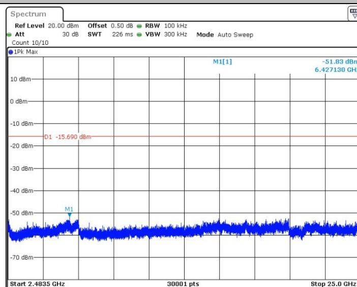
11B_Ant1_2437_2483.5~25000
