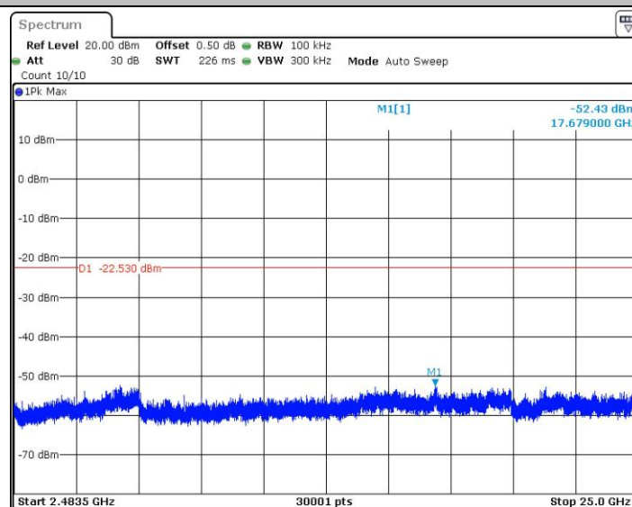
11N20SISO_Ant1_2437_2483.5~25000
