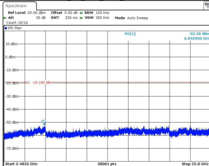
BLE_1M_Ant1_2480_2483.5~25000
