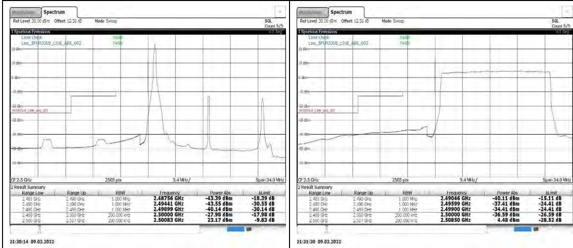
Band7-15MHz-16QAM-20825-1RB#0
