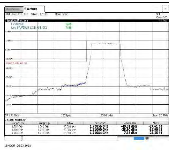
Band4-1.4MHz-QPSK-19957-6RB#0
