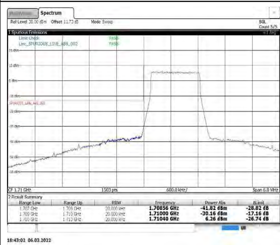
Band4-1.4MHz-16QAM-19957-6RB#0
