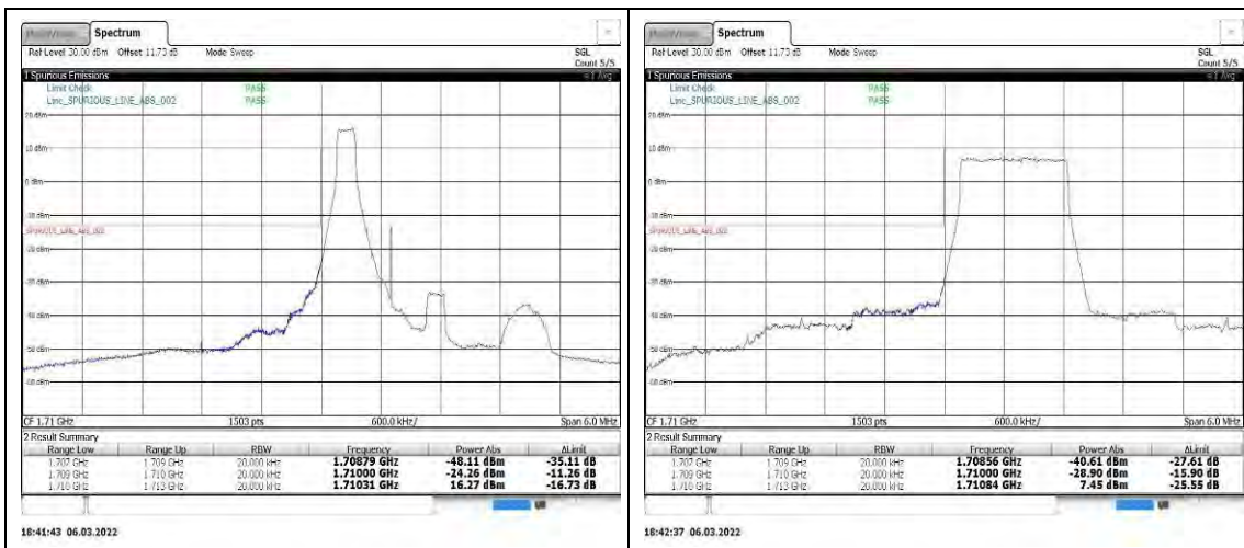
Band4-1.4MHz-QPSK-19957-1RB#0
