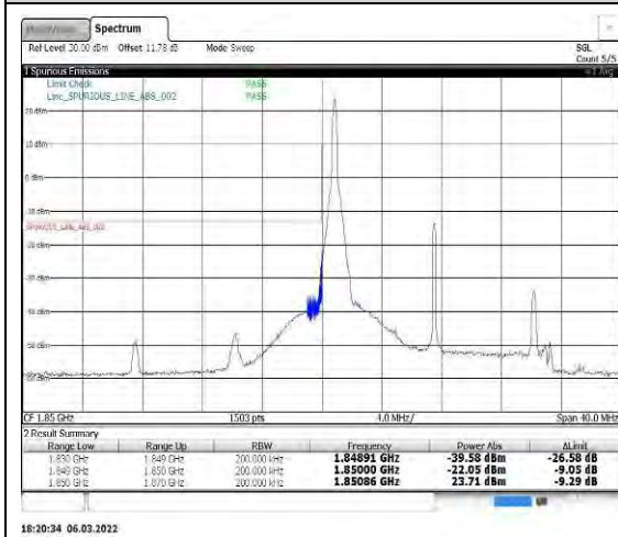
Band2-15MHz-QPSK-18675-1RB#0
