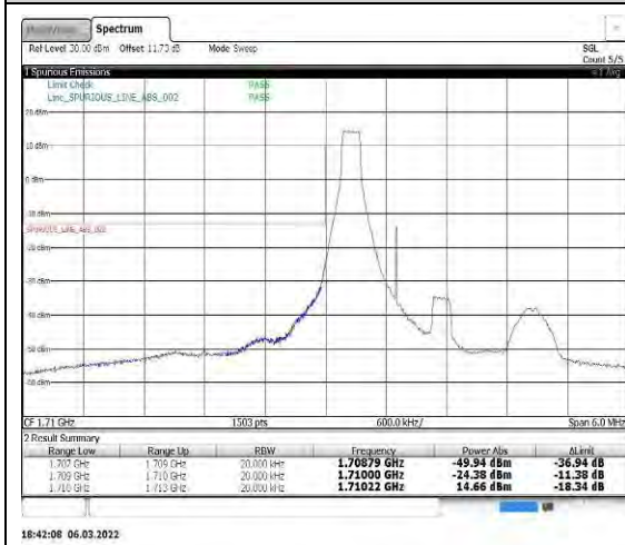
Band4-1.4MHz-16QAM-19957-1RB#0
