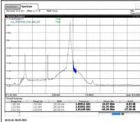
Band2-15MHz-QPSK-19125-1RB#74
