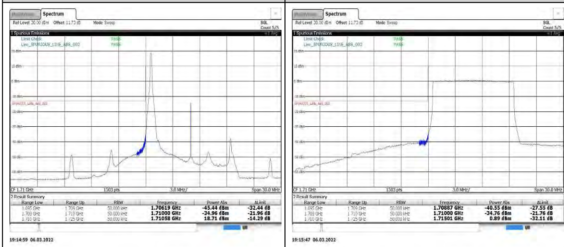
Band4-10MHz-16QAM-20000-1RB#0
