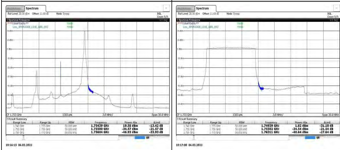
Band4-10MHz-QPSK-20350-1RB#49
