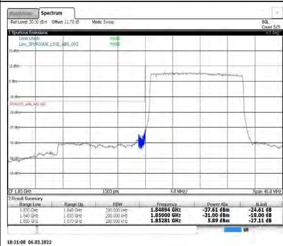
Band2-15MHz-QPSK-18675-75RB#0
