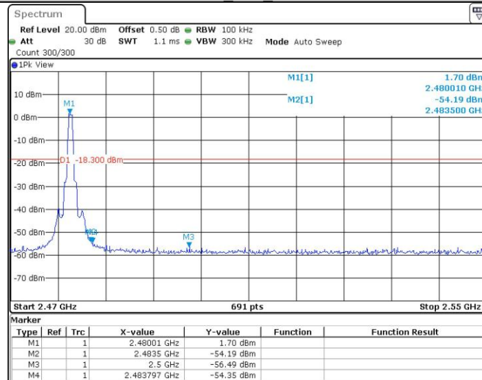
BLE_High_2480
