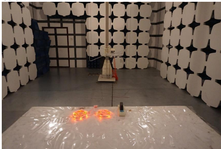
Radiated Emission
