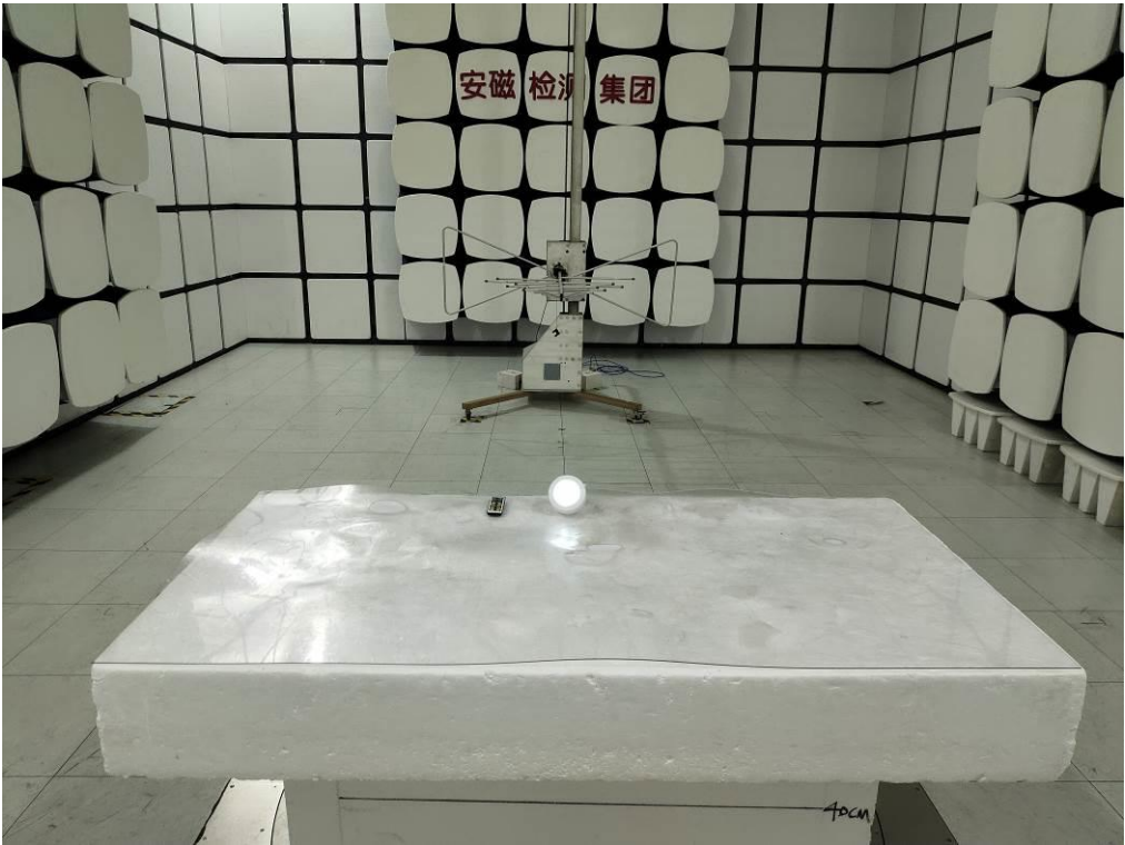
Photos of Radiation Emission Measurement
