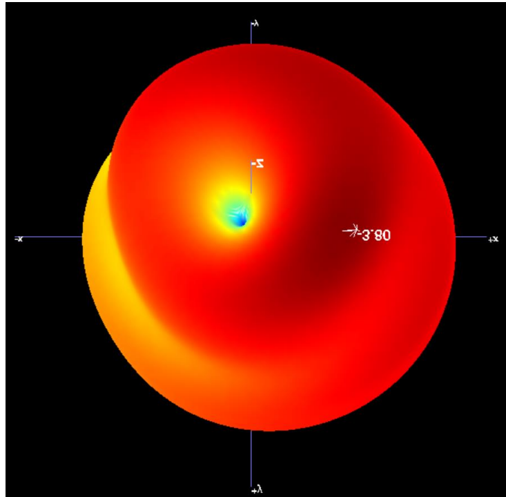
B1.1 3D Pattern for 433MHz
