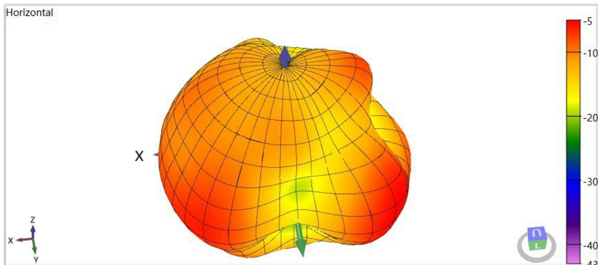
天线Antenna 2440MHz 3D-Horizontal Pattern
