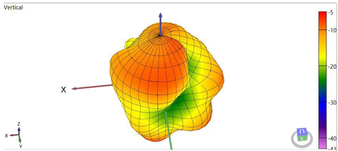
天线Antenna 2440MHz 3D-Vertical Pattern
