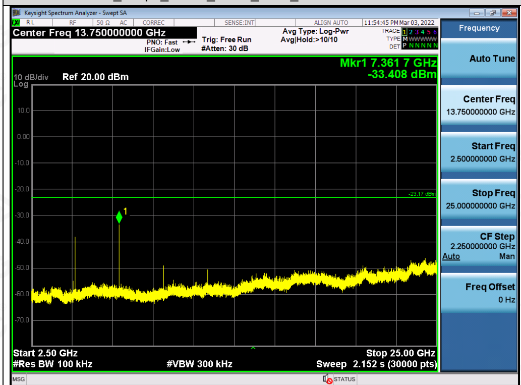
Test_Graph_GFSK_ANT1_2454_Higher Band Emissions
