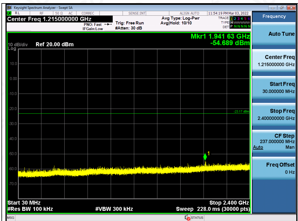
Test_Graph_GFSK_ANT1_2454_Lower Band Emissions
