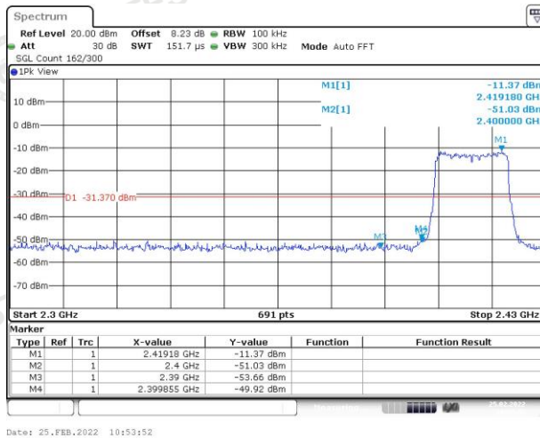
Left bandedge
