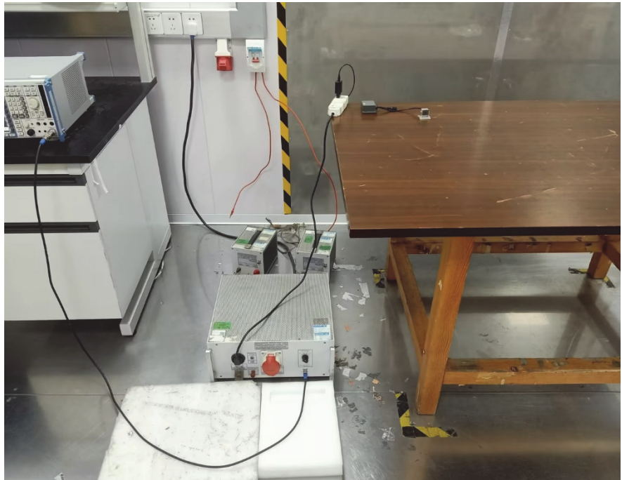
Conducted Emission Test Setup
