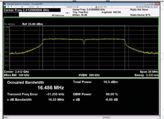
IEEE 802.11g_Channel 1_20MHz
