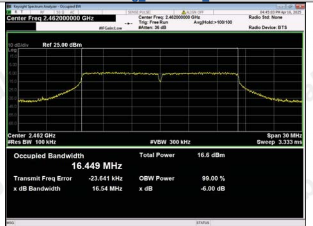
IEEE 802.11g_Channel 11_20MHz
