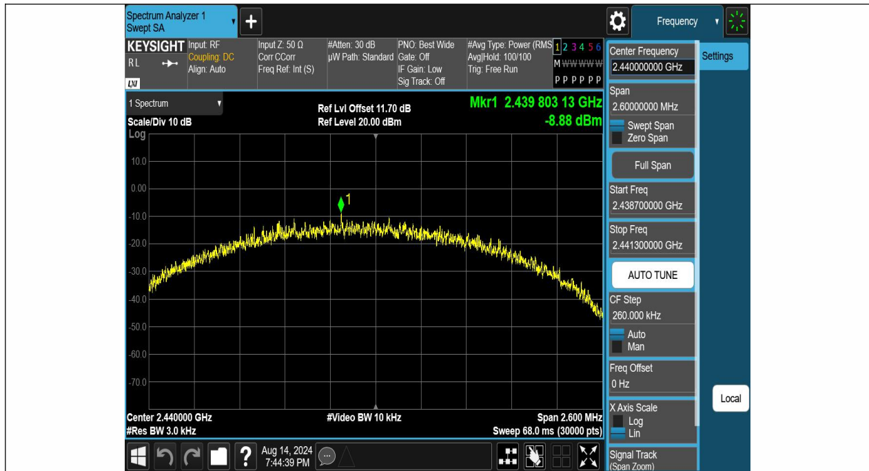
BLE_2M-Ant1-2440-PASS
