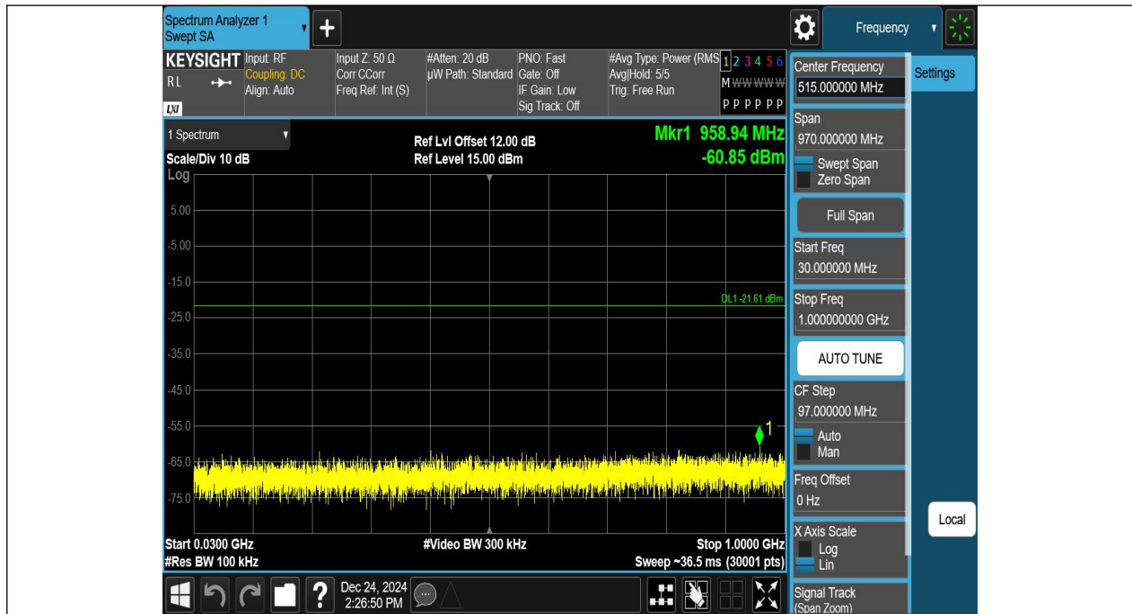
2.4GHz SRD_1M-Ant1-2440-30~1000-PASS
