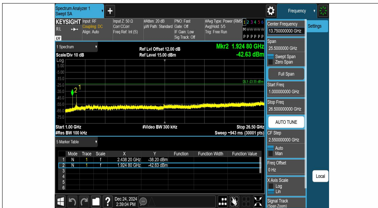
2.4GHz SRD_2M-Ant1-2440-1000~26500-PASS
