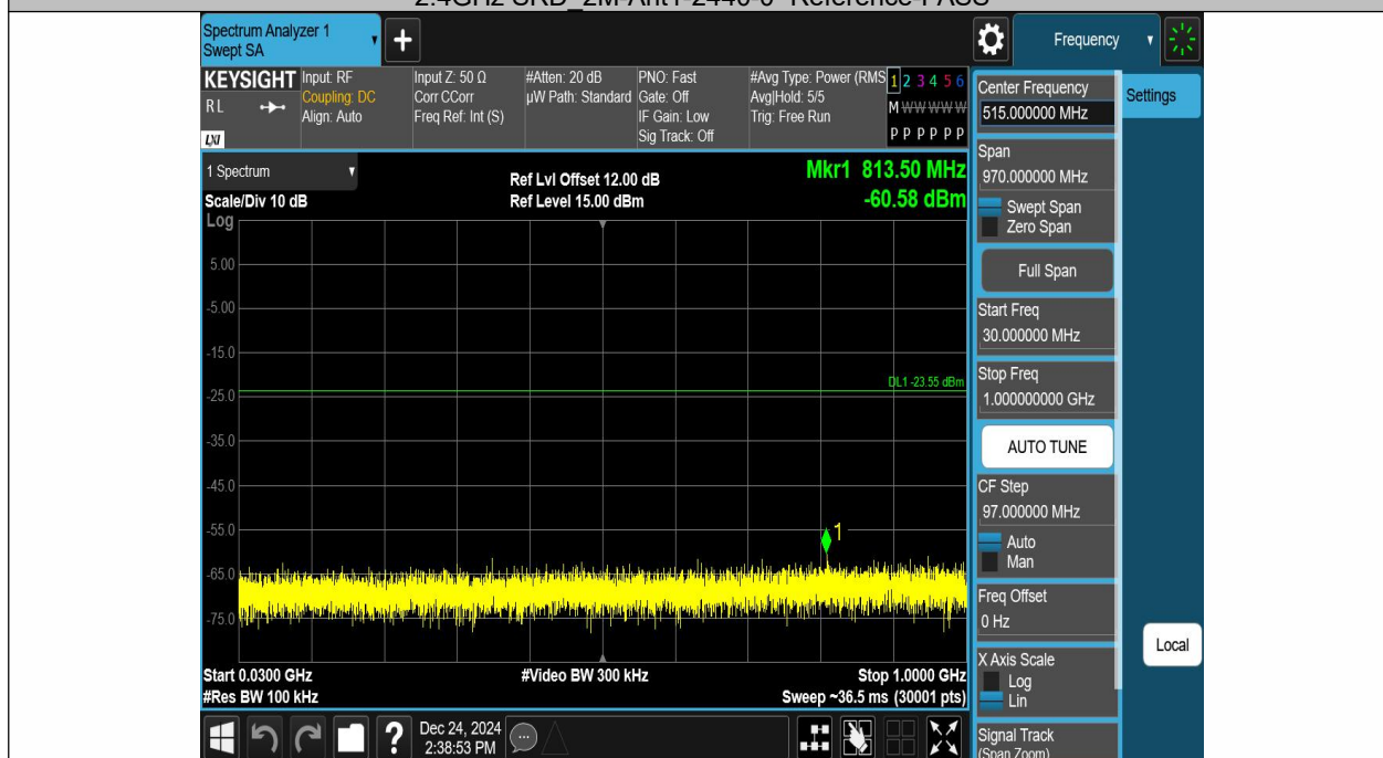
2.4GHz SRD_2M-Ant1-2440-30~1000-PASS
