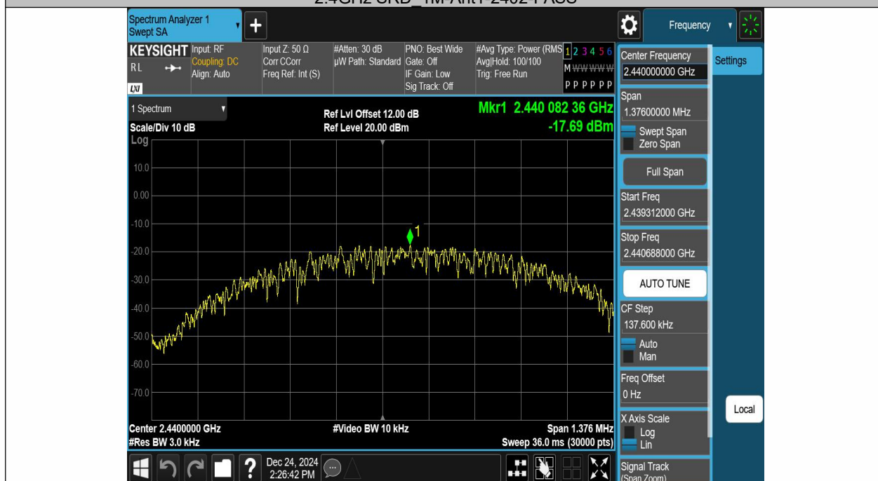
2.4GHz SRD_1M-Ant1-2440-PASS
