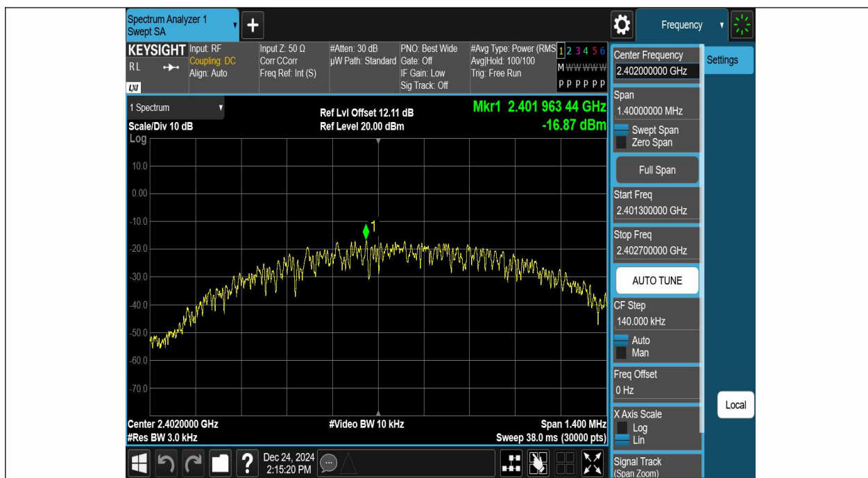
2.4GHz SRD_1M-Ant1-2402-PASS
