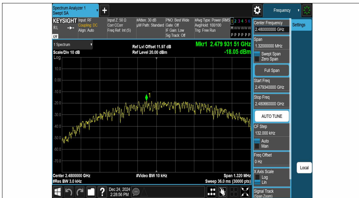
2.4GHz SRD 1M-Ant1-2480-PASS
