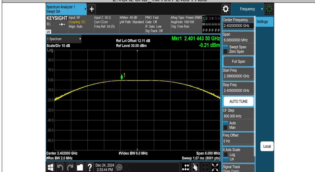
2.4GHz SRD 2M-Ant1-2402-PASS
