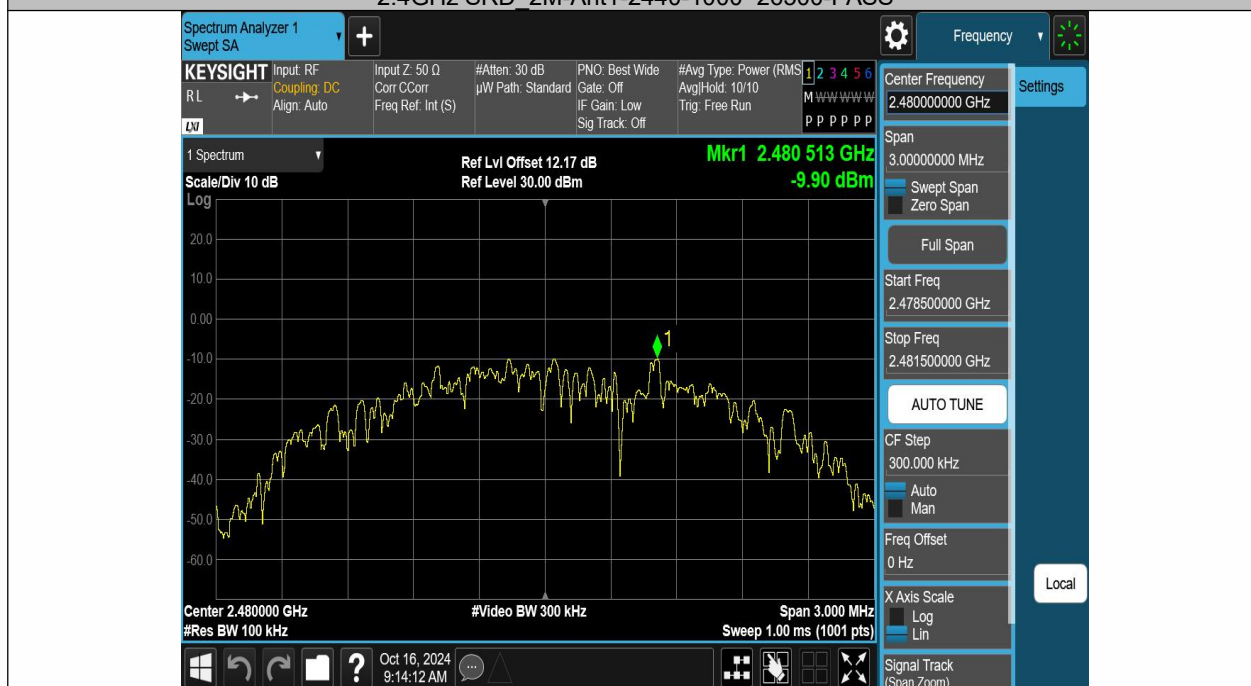
2.4GHz SRD_2M-Ant1-2480-0~Reference-PASS
