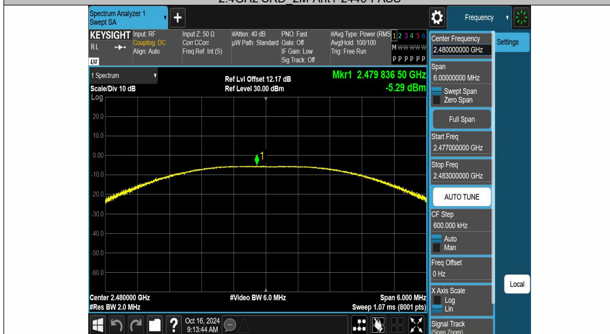
2.4GHz SRD 2M-Ant1-2480-PASS
