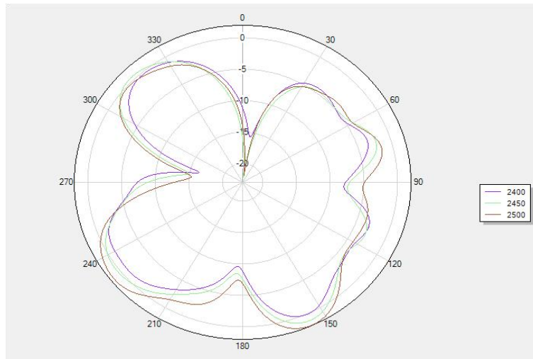
Phi 90 2D
