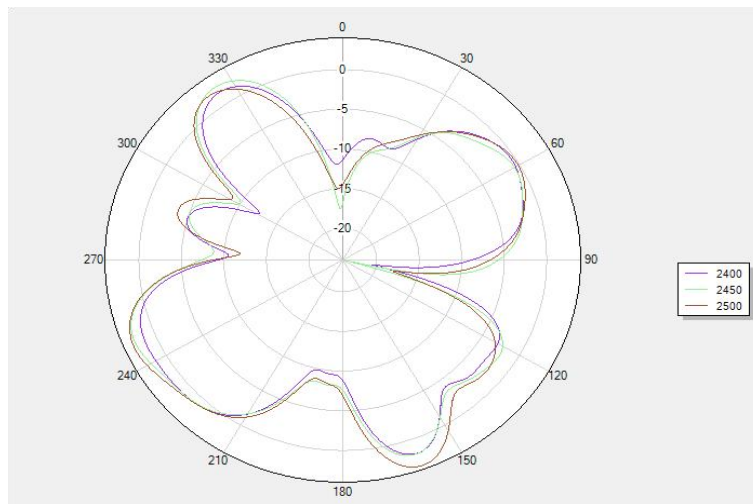
Theta 90 2D
