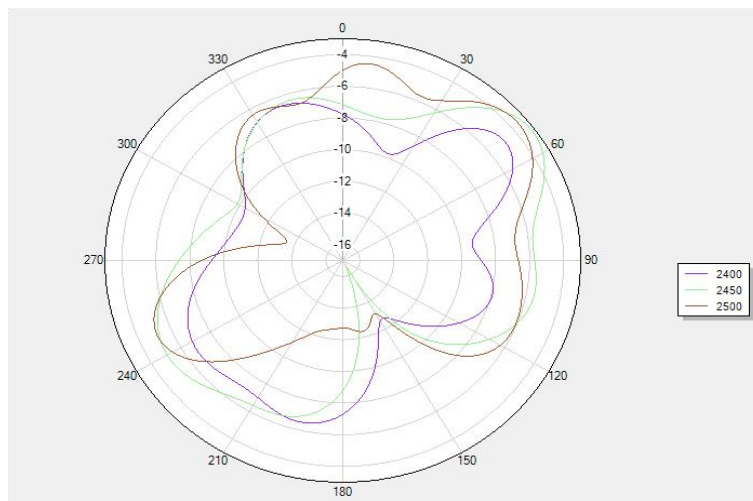
Theta 90 2D
