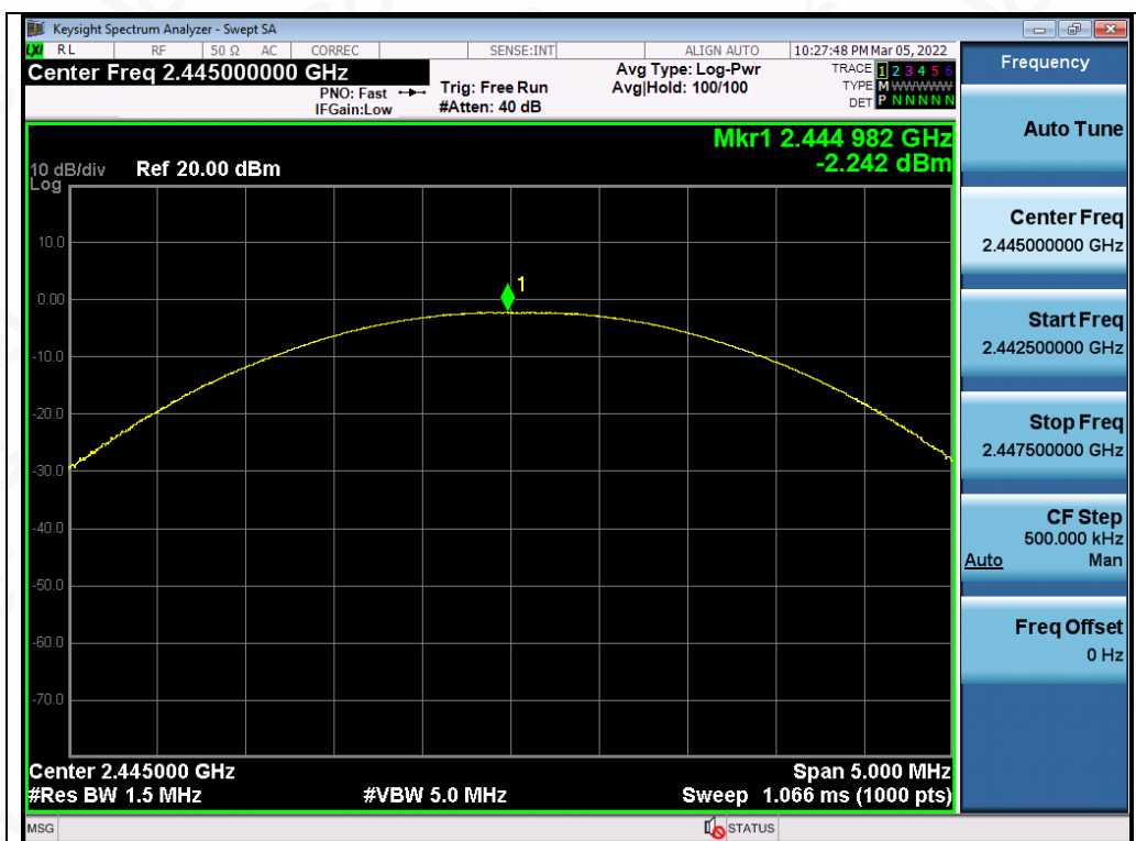
Test_Graph_GFSK_ANT1_2445_Peak Power
