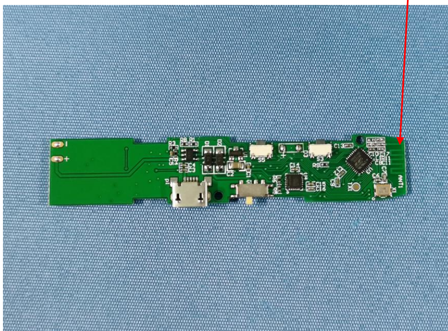
PCB Antenna
