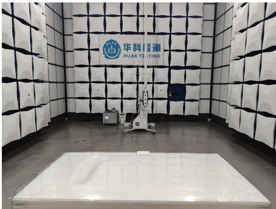
Model No.: QX-309FS Radiated Emissions
