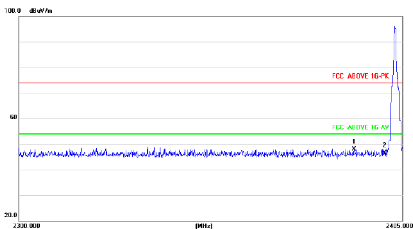
2401.25MHz Vertical
