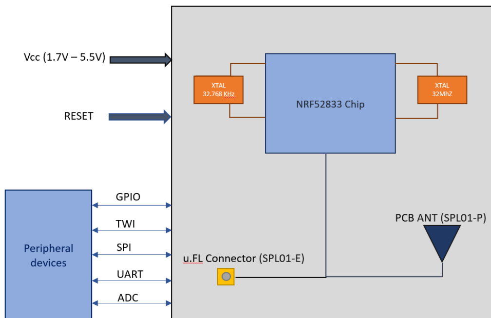
Figure 1: SPNYL01 Block diagram
