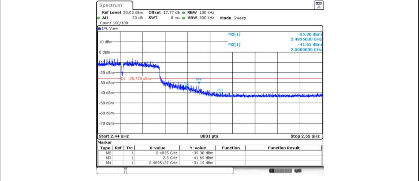
11N40SISO_Ant1_High_2452
