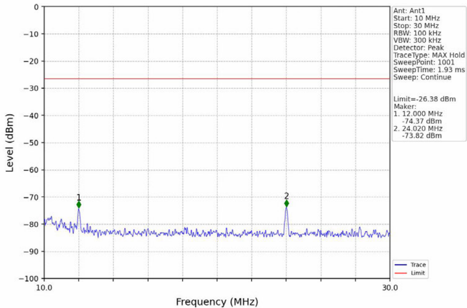
2.4g_MCH_2446MHz_Ant1_NTNV
