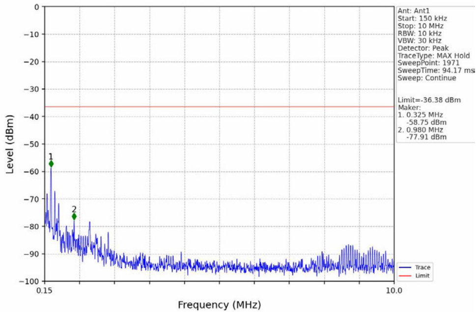
2.4g_MCH_2446MHz_Ant1_NTNV
