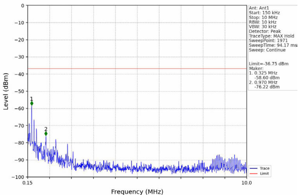
2.4g_LCH_2402MHz_Ant1_NTNV
