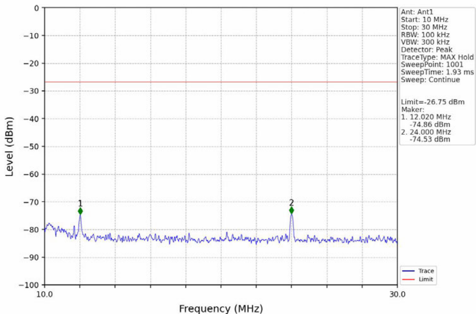
2.4g_LCH_2402MHz_Ant1_NTNV
