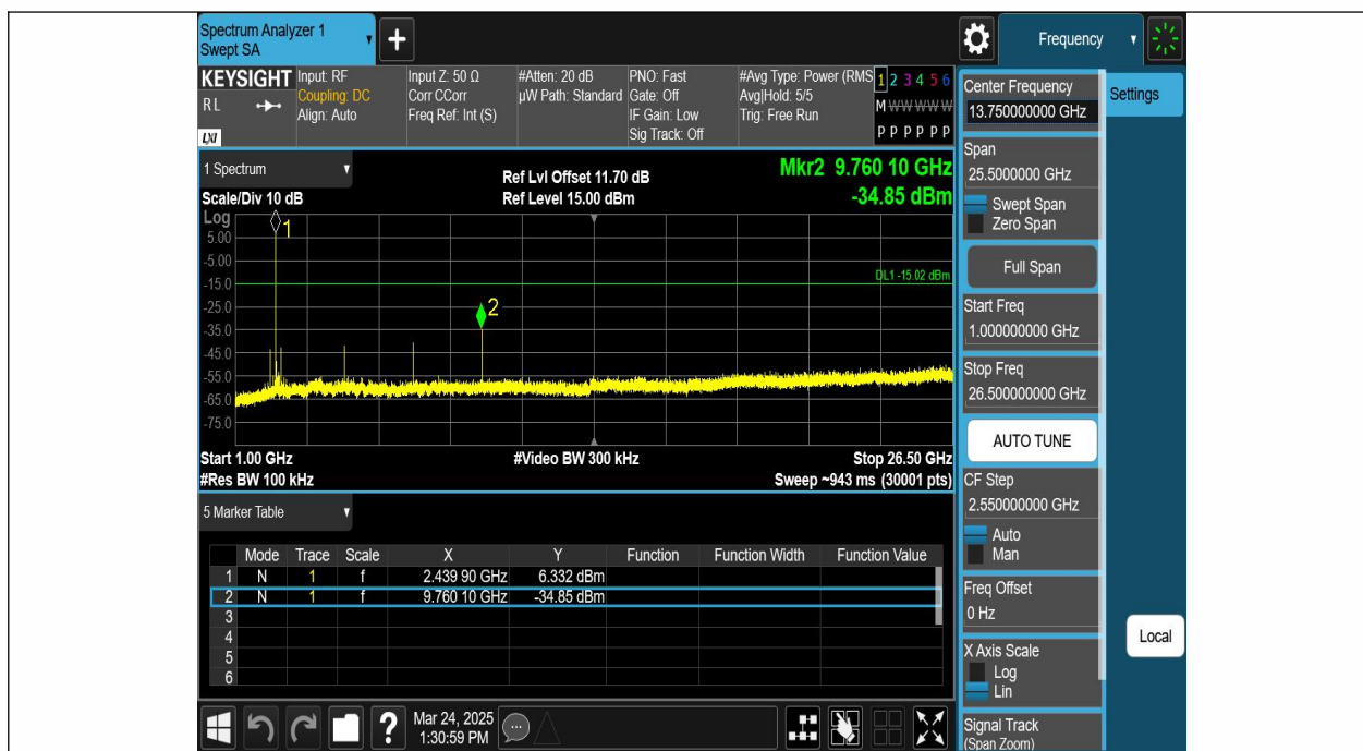
BLE_2M-Ant1-2440-1000~26500-PASS
