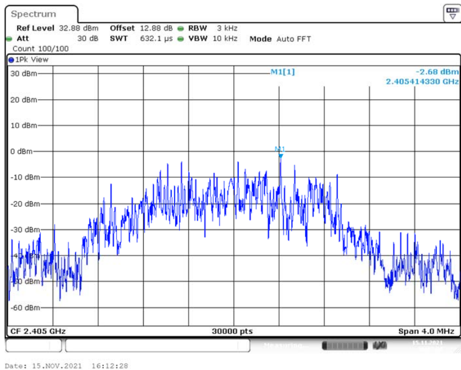
Power Spectral Density, Zigbee Low Channel
