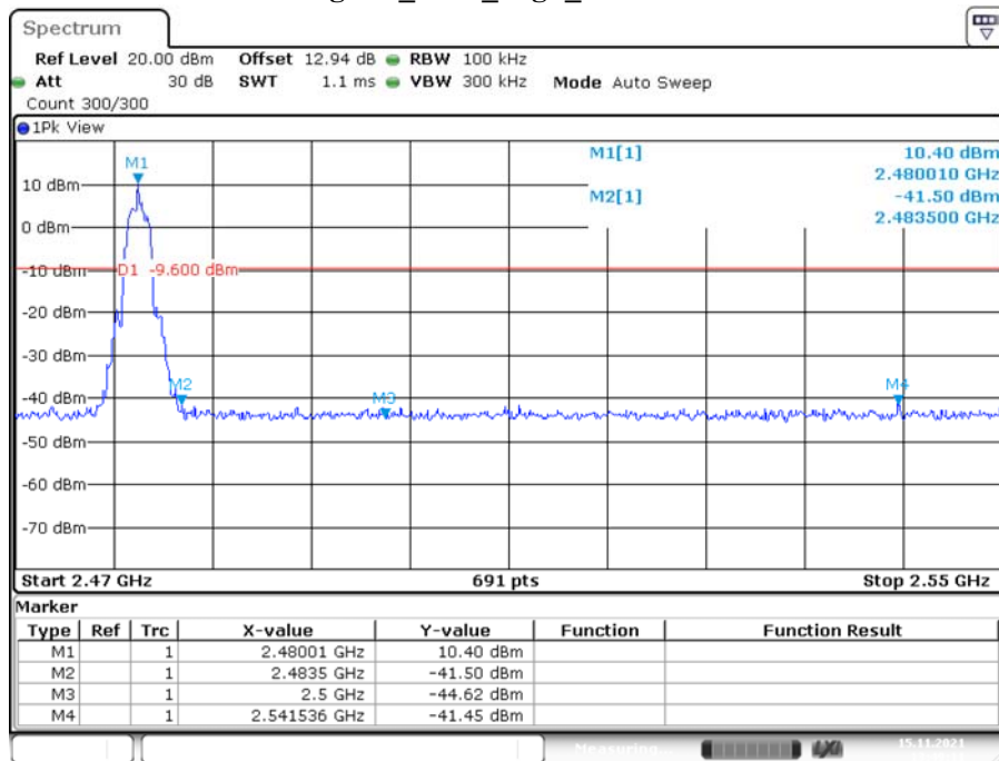
Zigbee_Ant1_High_2480MHz
