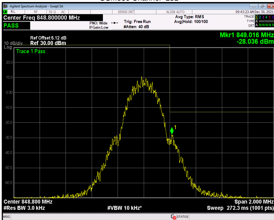
GSM850 Channel=251
