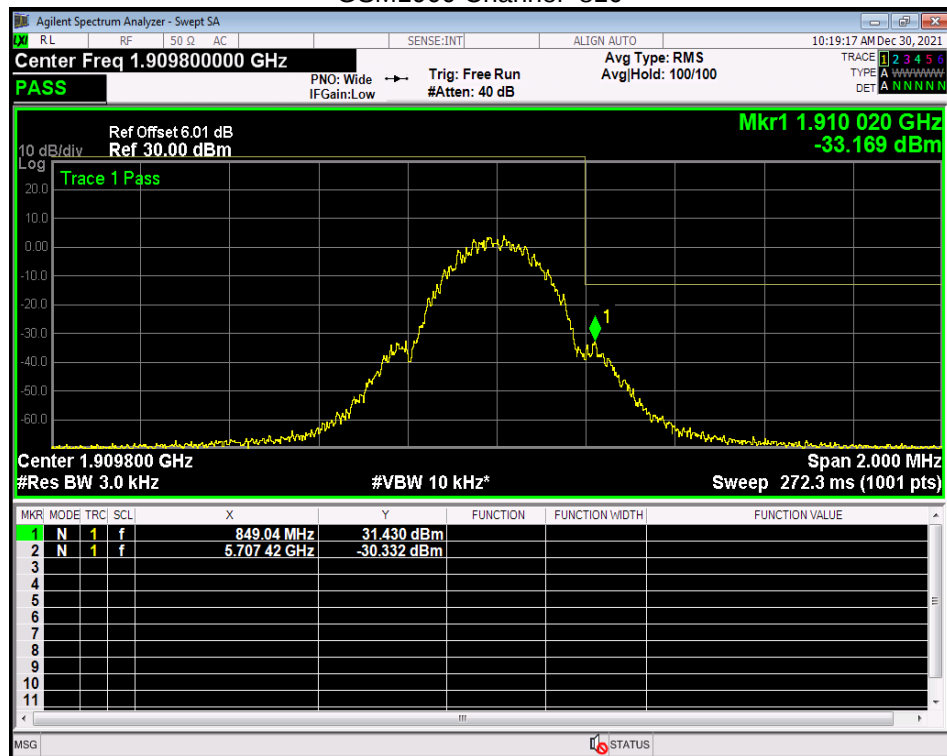
GSM1900 Channel=810
