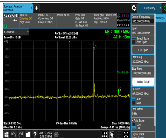
Band12-5MHz-16QAM-23155-1RB#0-Range3:30~1000MHz
