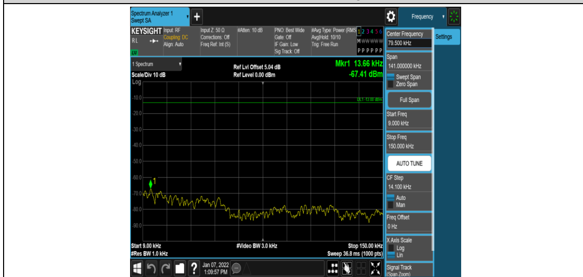
Band2-10MHz-QPSK-19150-1RB#0-Range1:0.009~0.15MHz
