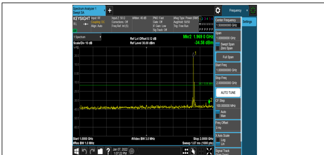
Band2-10MHz-16QAM-18650-1RB#0-Range4:1000~2000MHz
