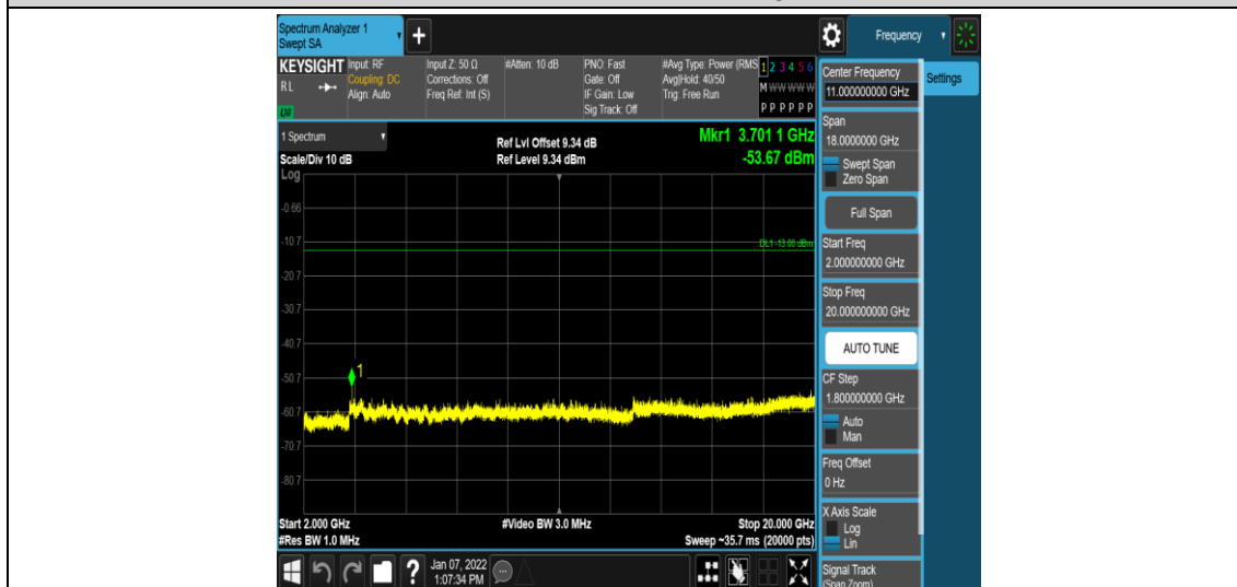
Band2-10MHz-16QAM-18650-1RB#0-Range5:2000~20000MHz
