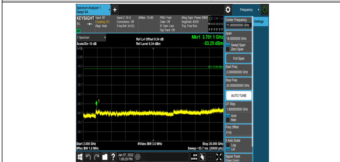
Band2-10MHz-QPSK-18650-1RB#0-Range5:2000~20000MHz
