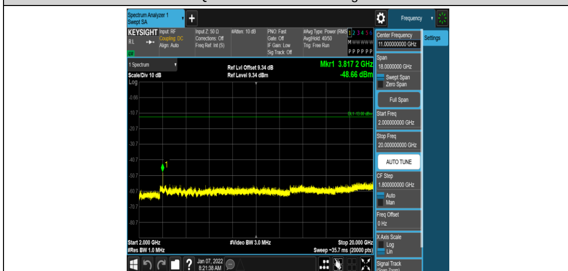
Band2-1.4MHz-QPSK-19193-1RB#0-Range5:2000~20000MHz
