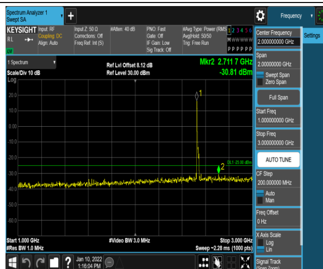
Band7-20MHz-16QAM-21100-1RB#0-Range4:1000~3000MHz
