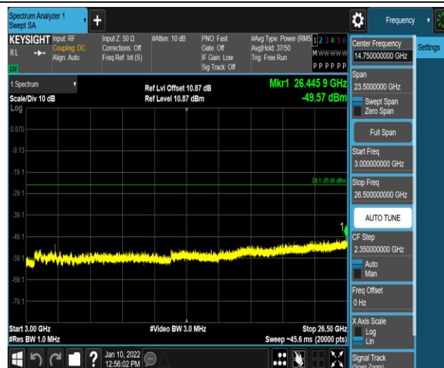
Band7-15MHz-QPSK-21375-1RB#0-Range5:3000~26500MHz
