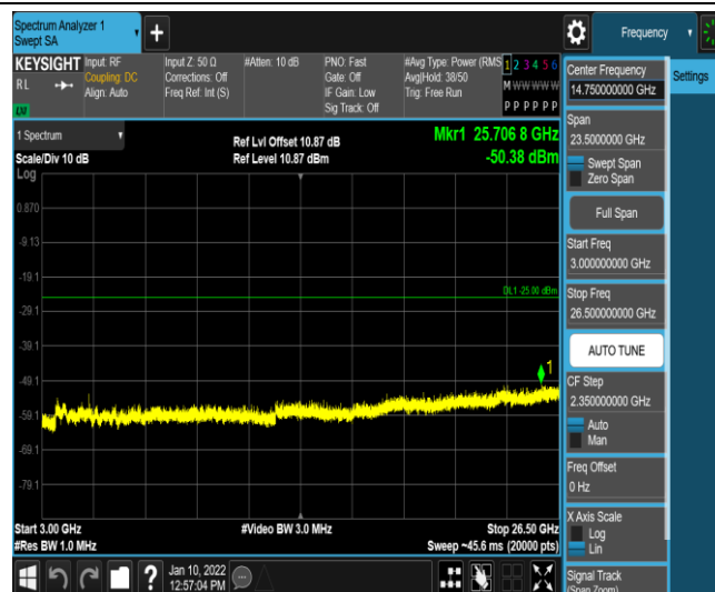
Band7-15MHz-16QAM-21375-1RB#0-Range5:3000~26500MHz
