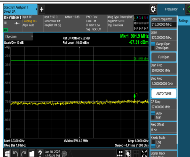
Band7-15MHz-QPSK-21100-1RB#0-Range3:30~1000MHz
