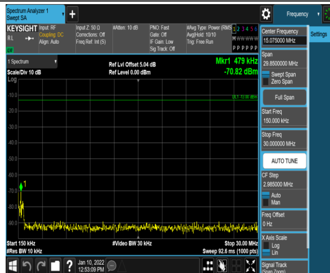
Band7-15MHz-QPSK-21100-1RB#0-Range2:0.15~30MHz
