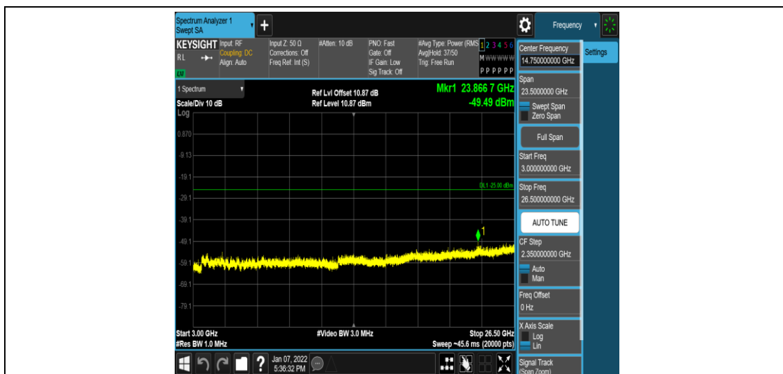
Band7-5MHz-16QAM-21425-1RB#0-Range5:3000~26500MHz
