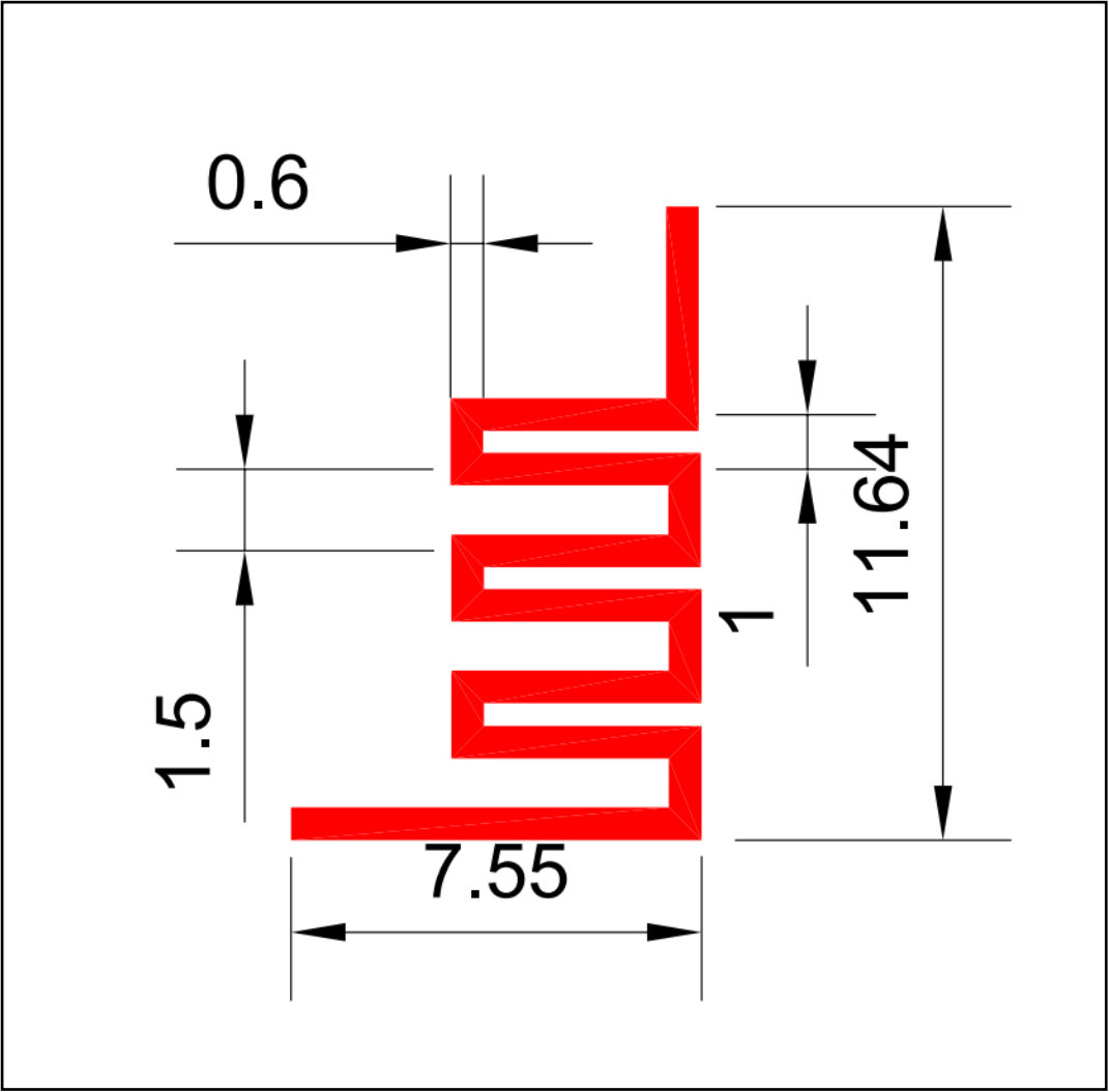
产品规格图(Antenna Specification chart)
