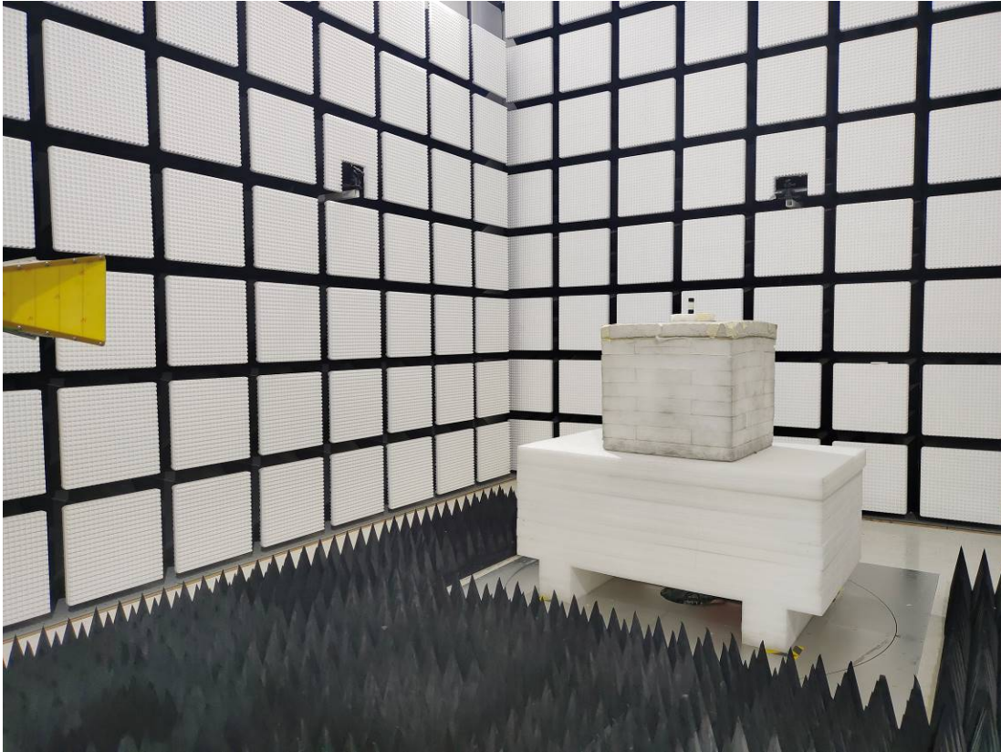
Radiated Emission Above 18GHz - 26.5GHz View
