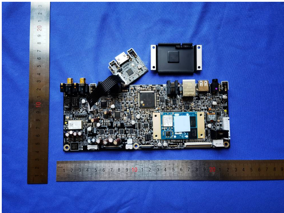
Fig 20. Digital board view 2
