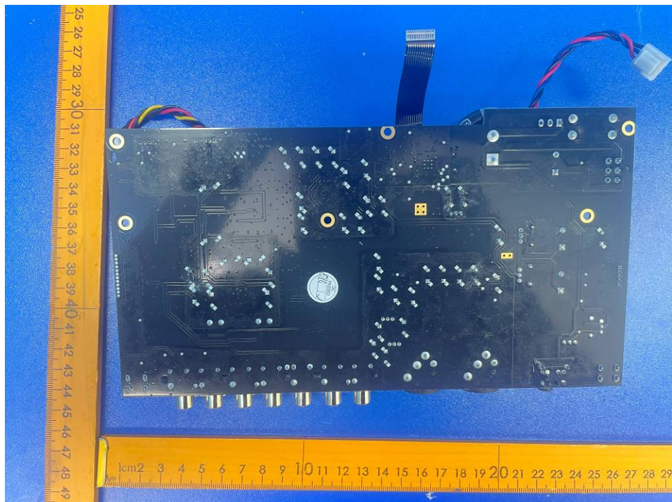
Fig 18. AMP board view 2
