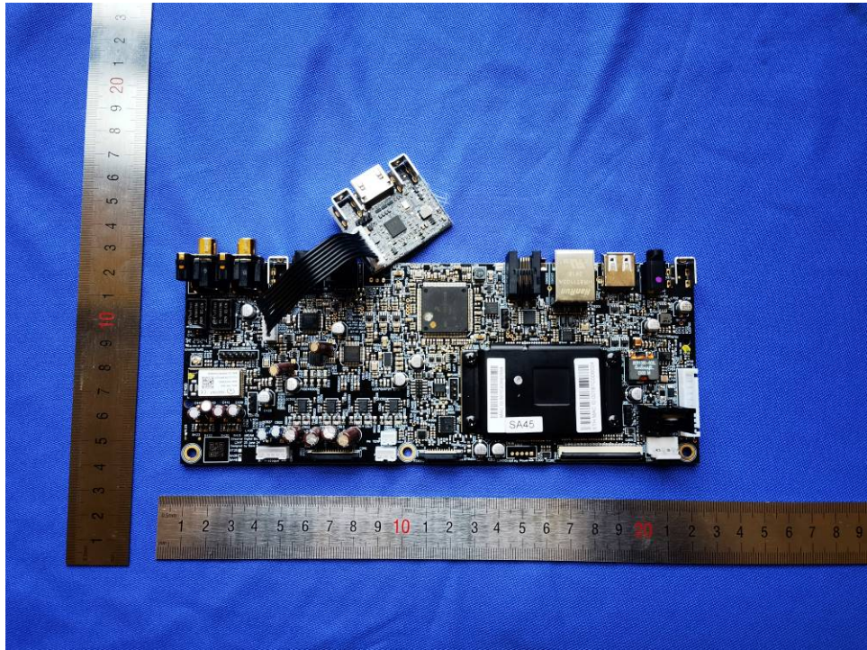
Fig 19. Digital board view 1
