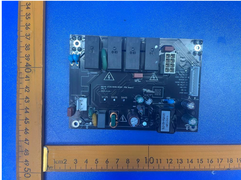
Fig 15. Power board view 1
