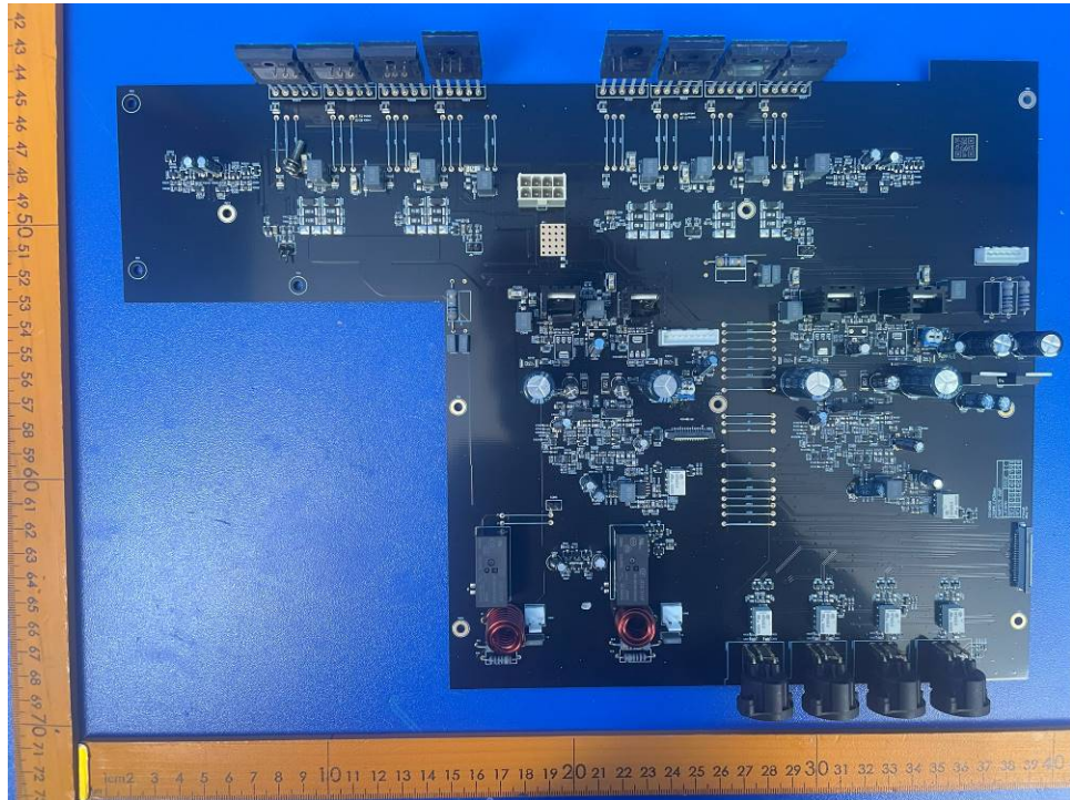
Fig 13. FPC isolation board view 1
