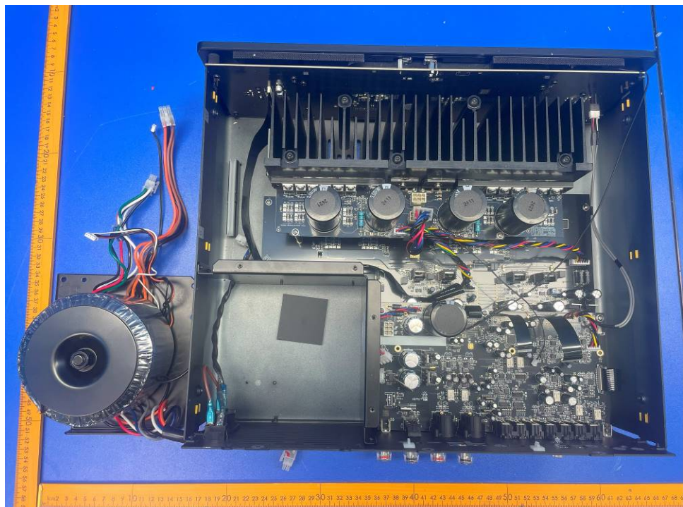
Fig 6. Internal view 4
