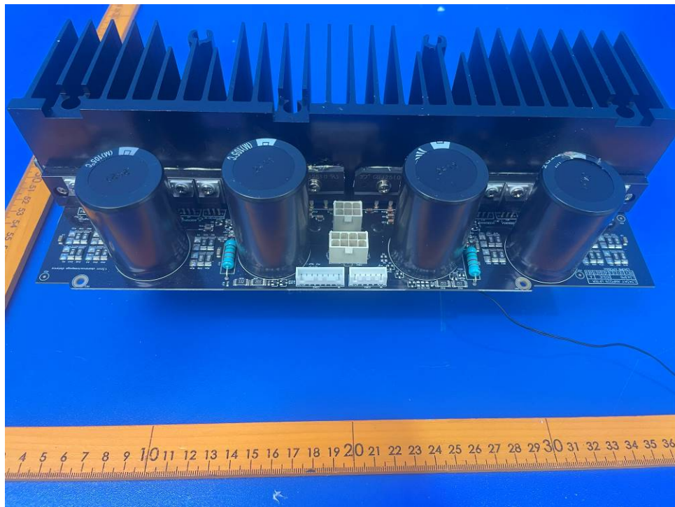
Fig 11. Lifter board view 1
