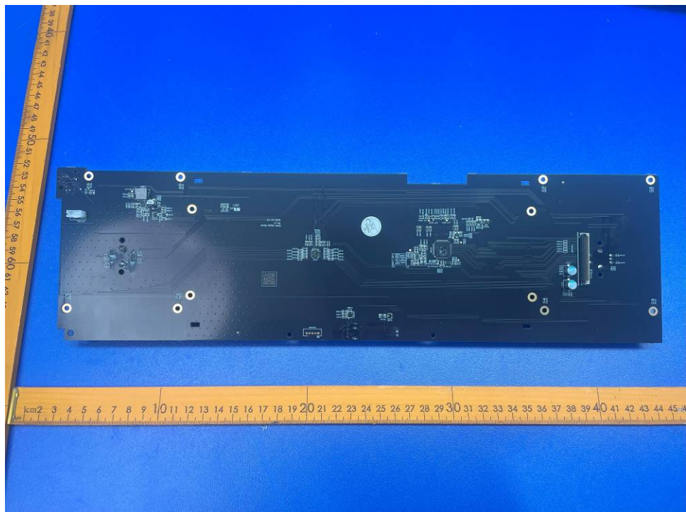
Fig 22. Display and knob board view 1
