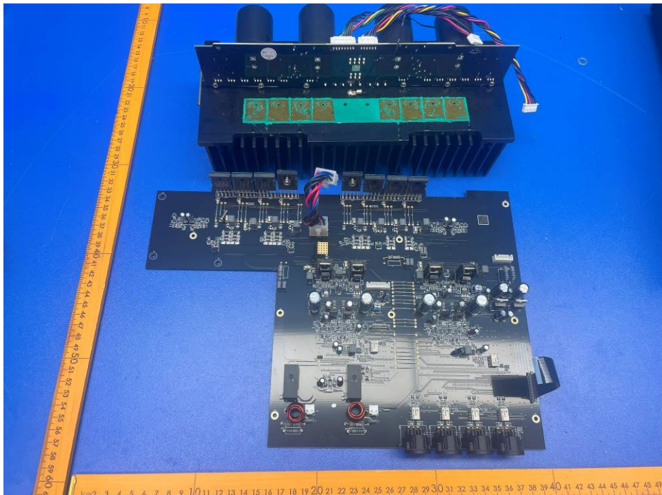
Fig 10. Internal view 8
