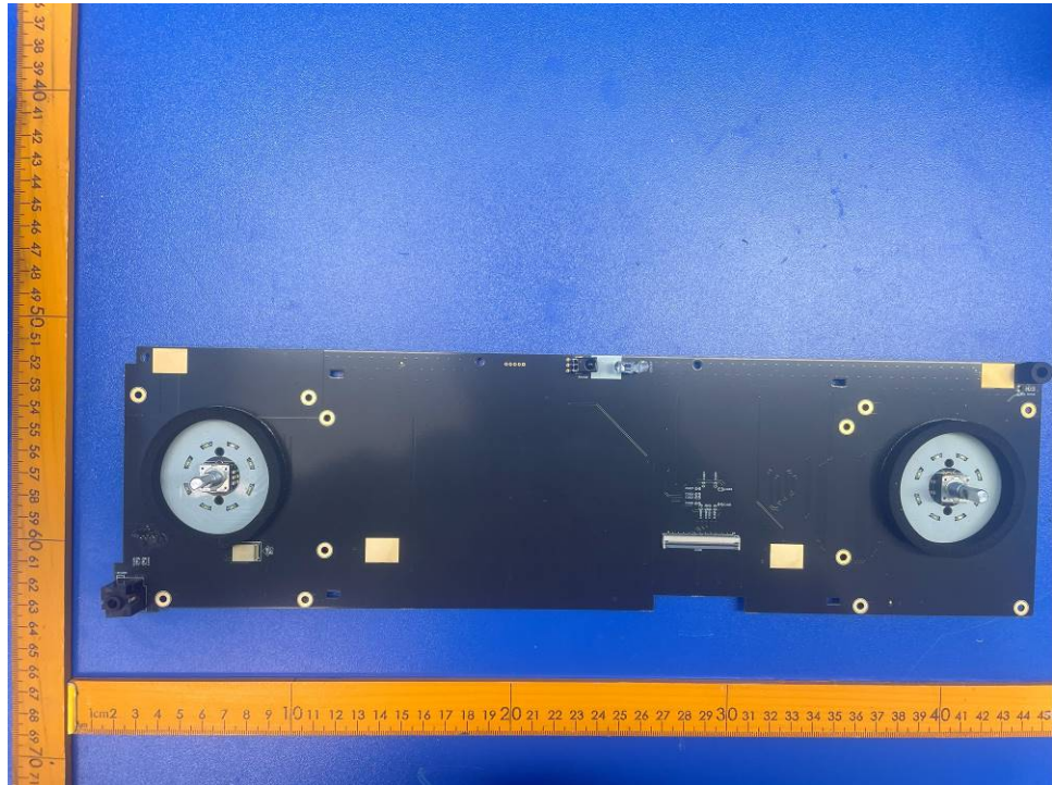
Fig 23. Display and knob board view 2
