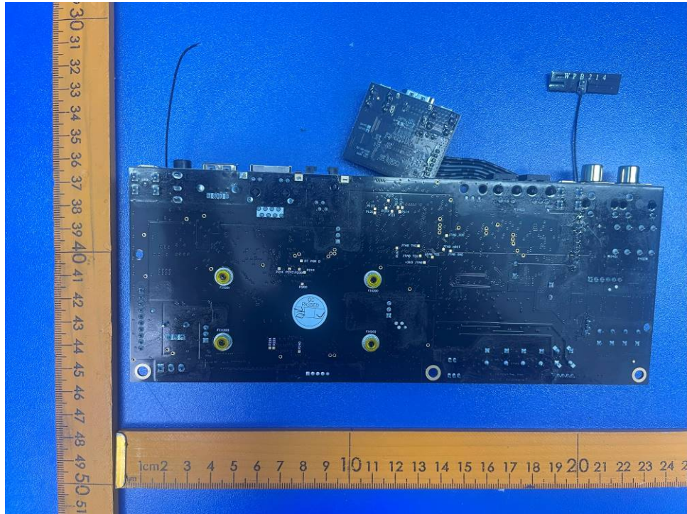
Fig 21. Digital board view 3
