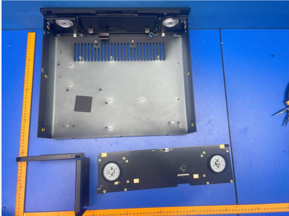
Fig 9. Internal view 7
