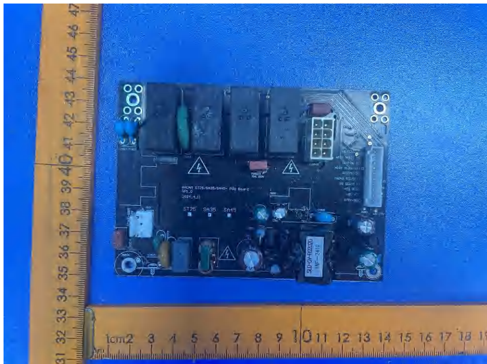
Fig 10. Power board view 1
