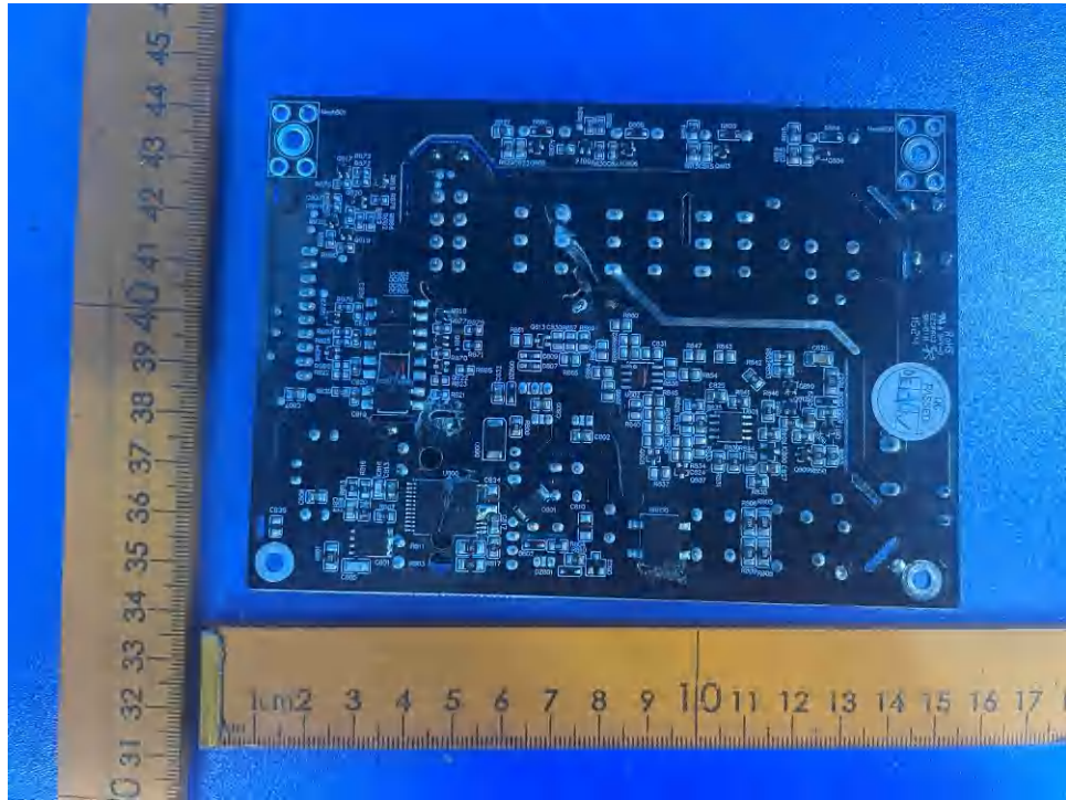
Fig 11. Power board view 2
