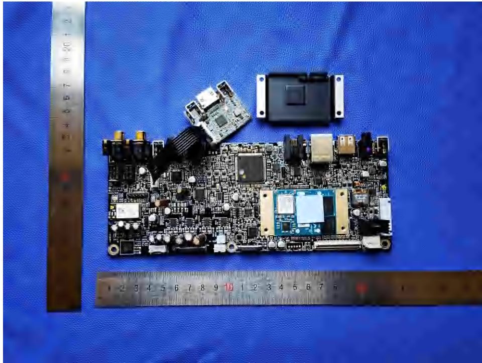
Fig 13. Digital board view 2
