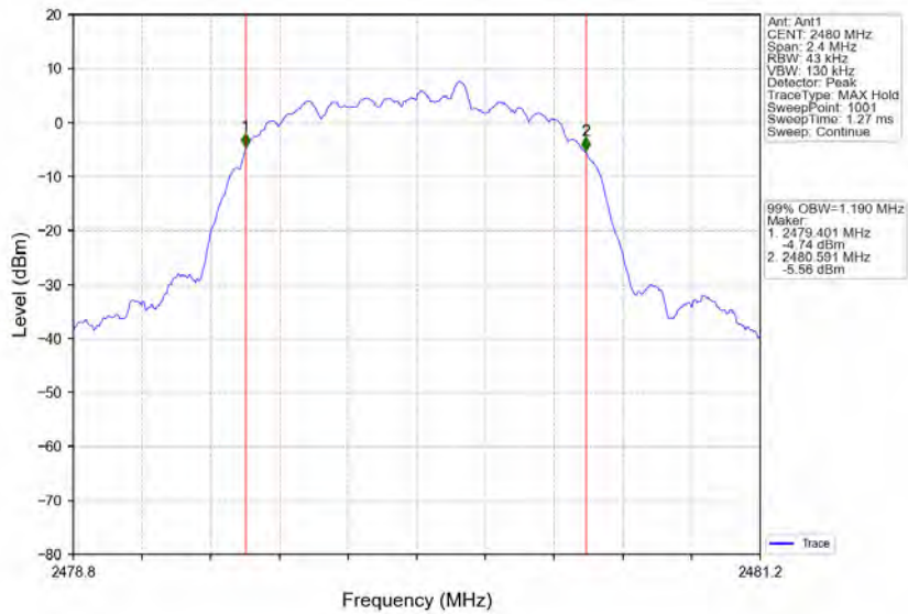
8DPSK_3DH5_HCH_2480MHz_Ant1_NTNV
