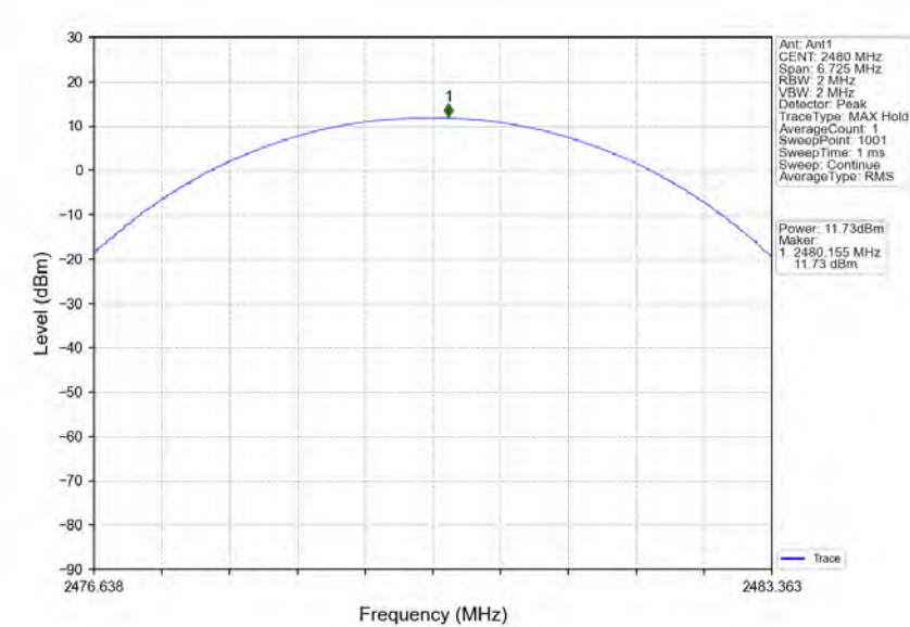
Pi/4DQPSK_2DH5_HCH_2480MHz_Ant1_NTNV
