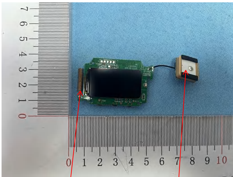
433.92MHz RX ANT
