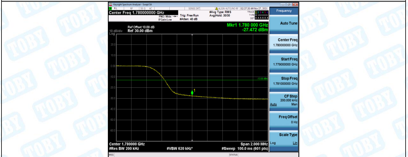
Band66-10MHz-16QAM-132022-50RB#0
