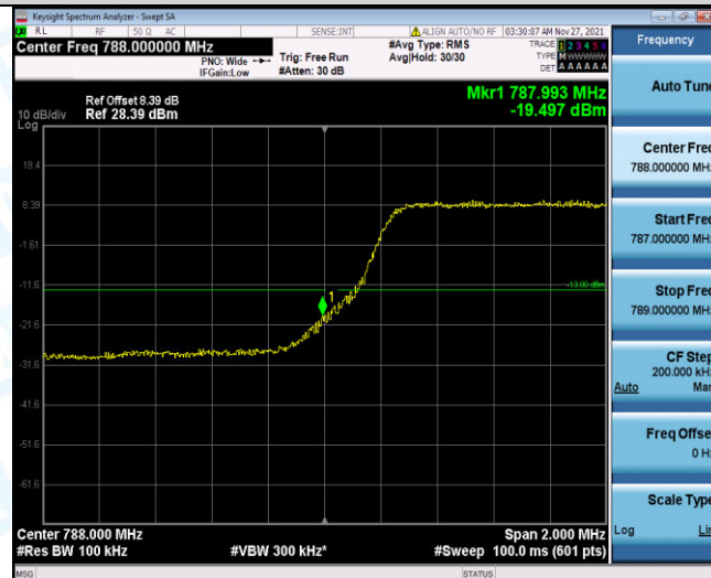
Band14-5MHz-16QAM-23355-25RB#0
