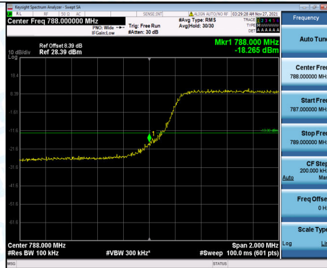
Band14-5MHz-QPSK-23355-25RB#0
