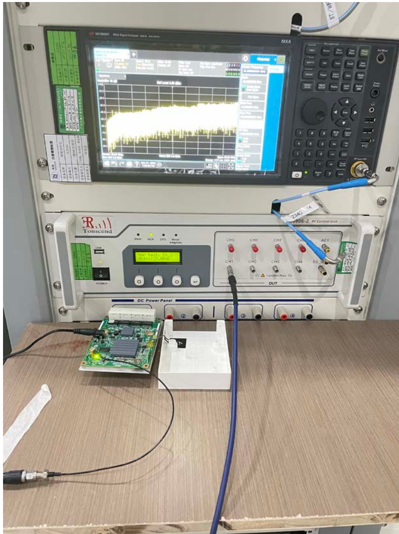
Setup photo
