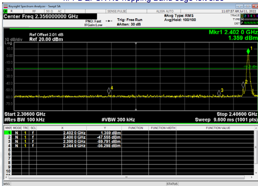
\pi/4 -DQPSK No-hopping Band edge-left side
