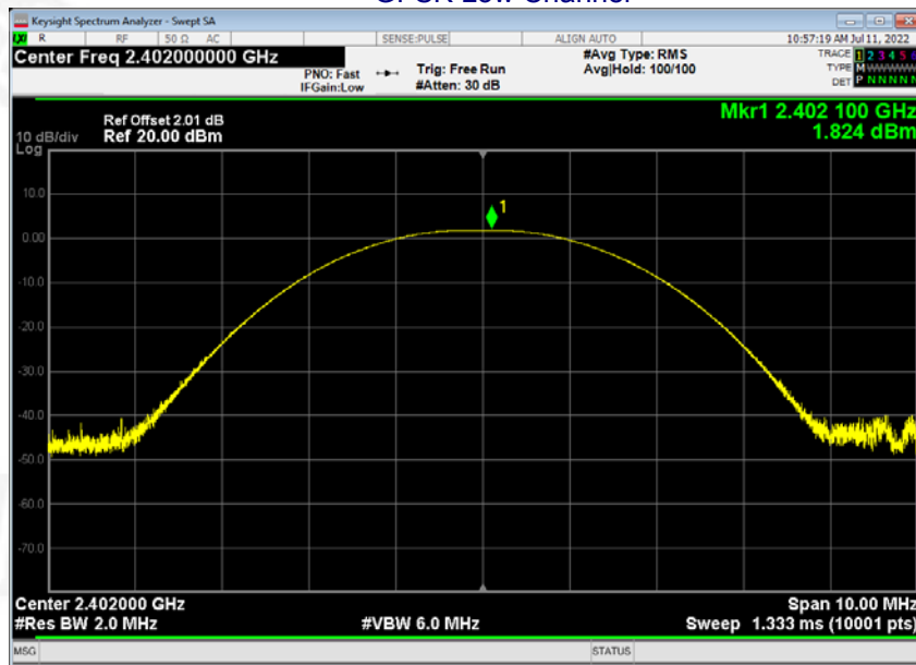
GFSK Low Channel
