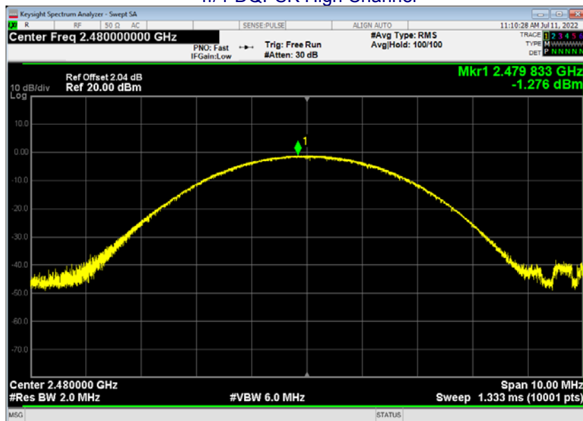
\pi/4 -DQPSK High Channel
