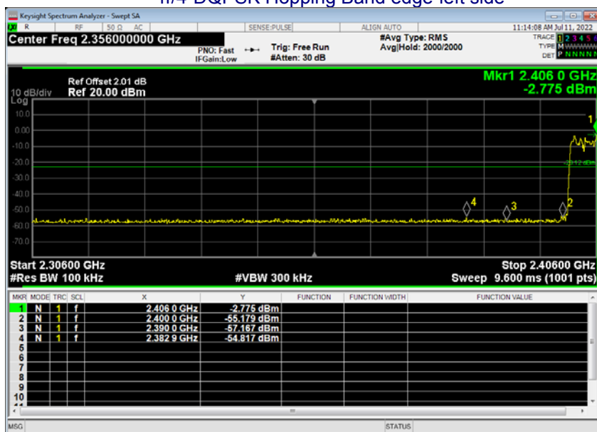
\pi/4 -DQPSK Hopping Band edge-left side
