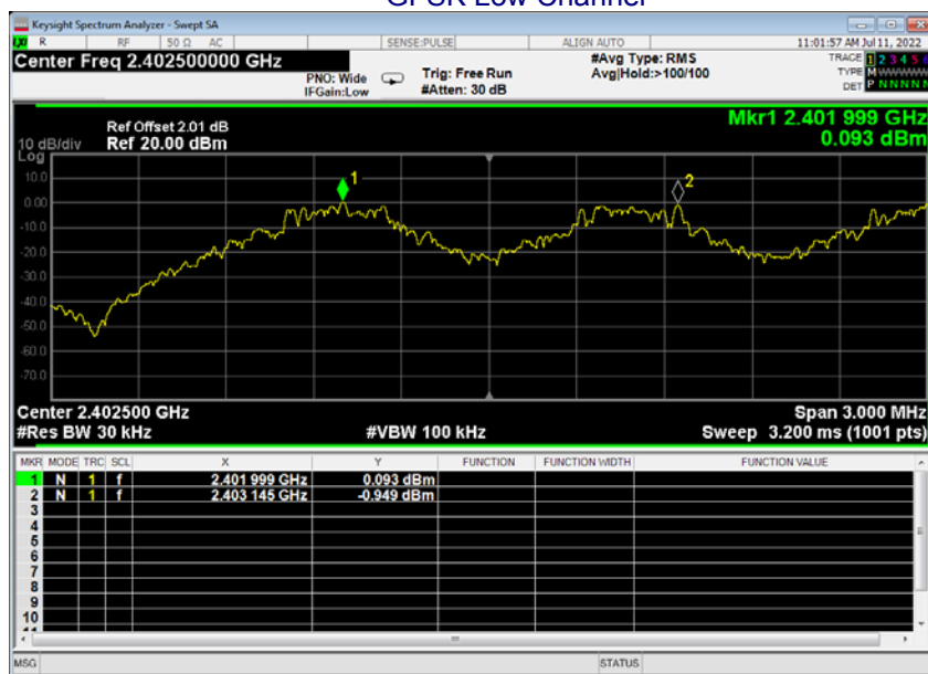
Test plots GFSK Low Channel
