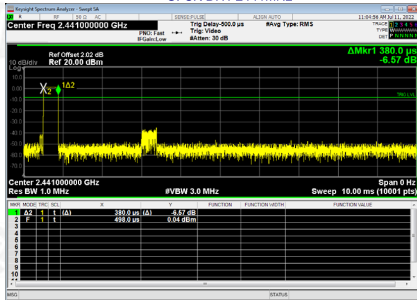
GFSK DH1 2441MHz
