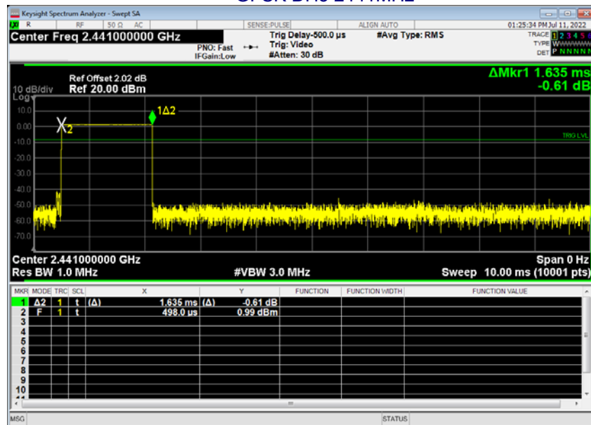
GFSK DH3 2441MHz
