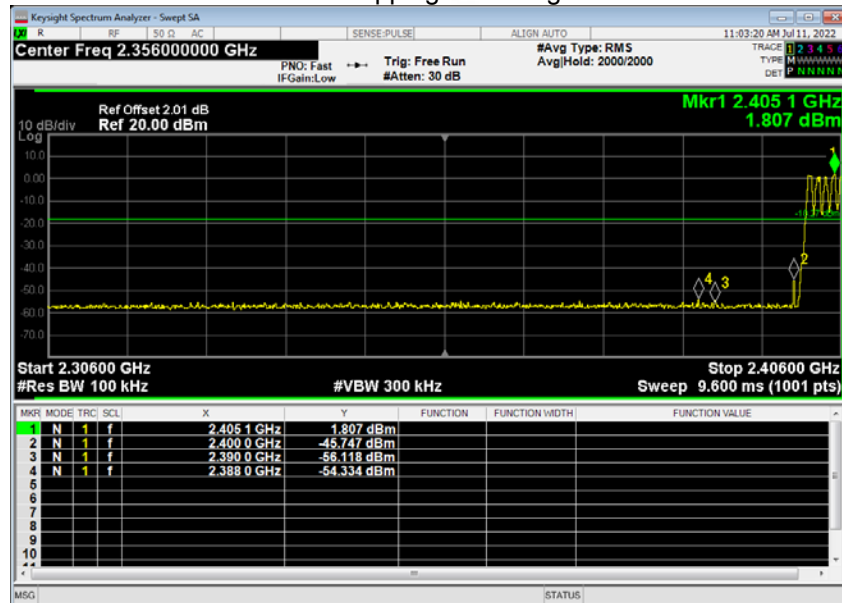
GFSK Hopping Band edge-left side
