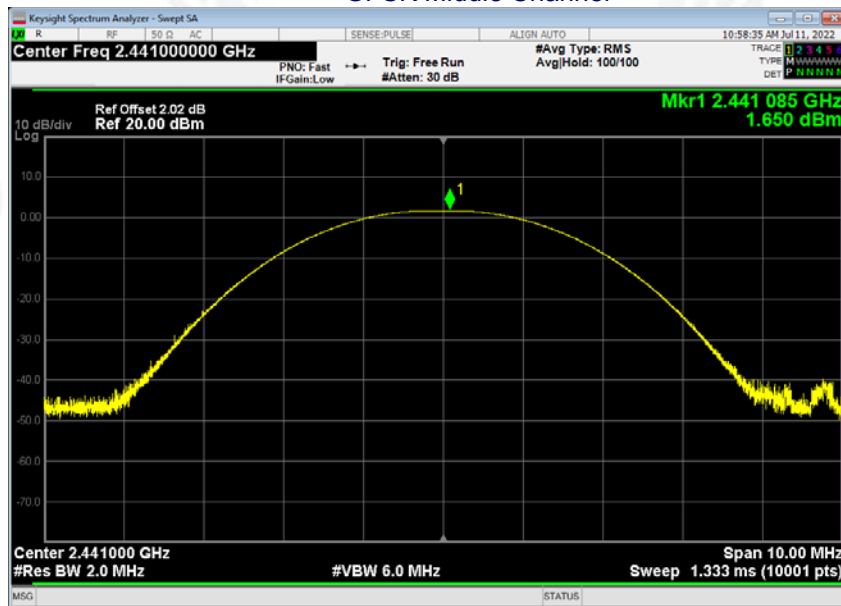
GFSK Middle Channel
