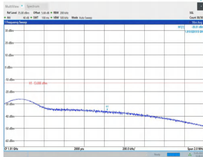
Band2-15MHz-QPSK-19125-1RB#74
