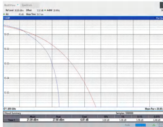
Band2-10MHz-16QAM-18650-50RB#0
