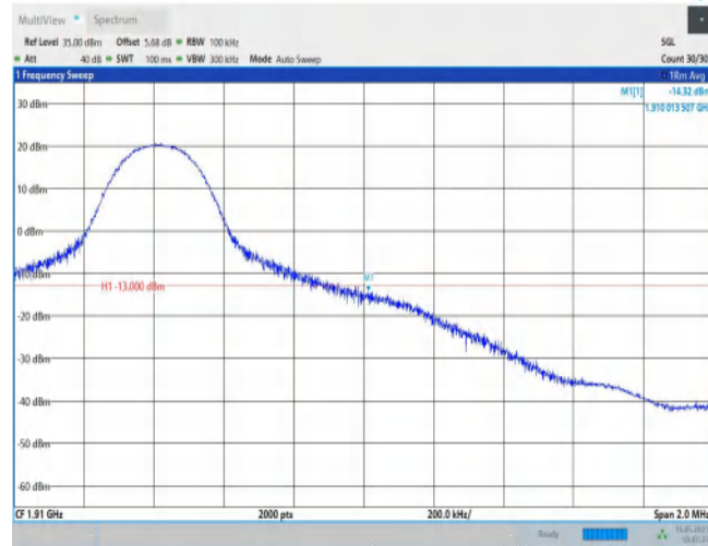
Band2-10MHz-QPSK-19150-50RB#0
