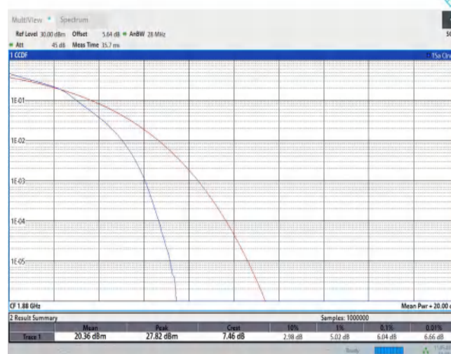
Band2-5MHz-16QAM-19175-1RB#0
