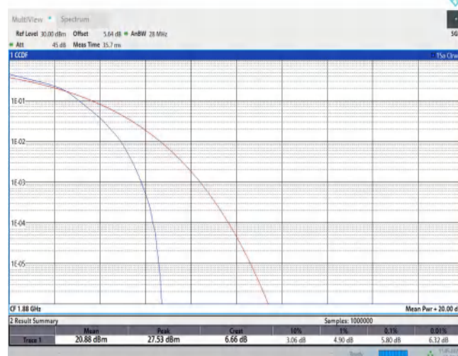
Band2-1.4MHz-16QAM-18900-6RB#0
