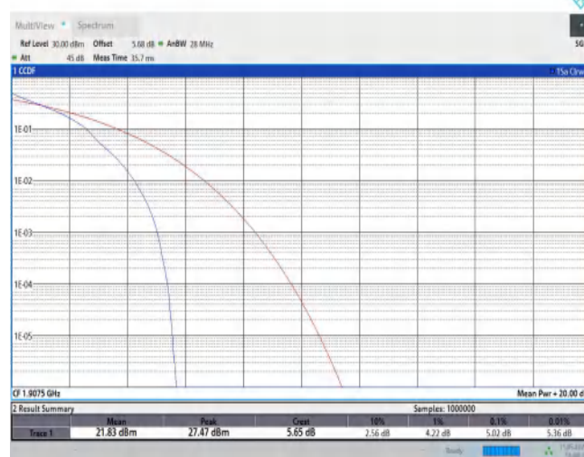
Band2-5MHz-QPSK-19175-25RB#0
